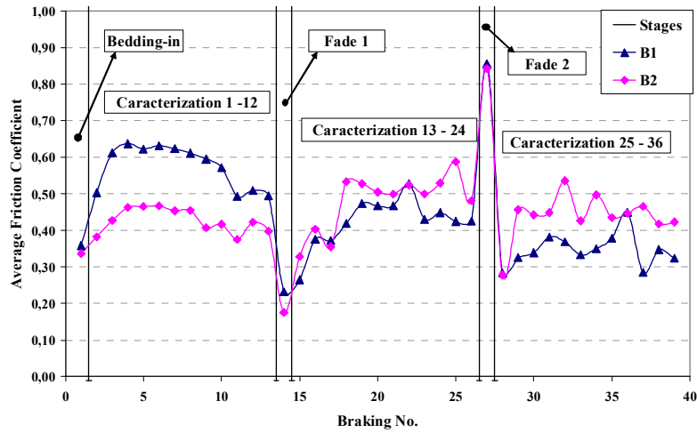
Figure 6 – Average Fiction coefficient for samples B1 and B2.
