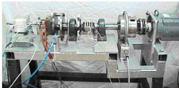
Figure 1 - Braking tribometer designed by UFRGS.
