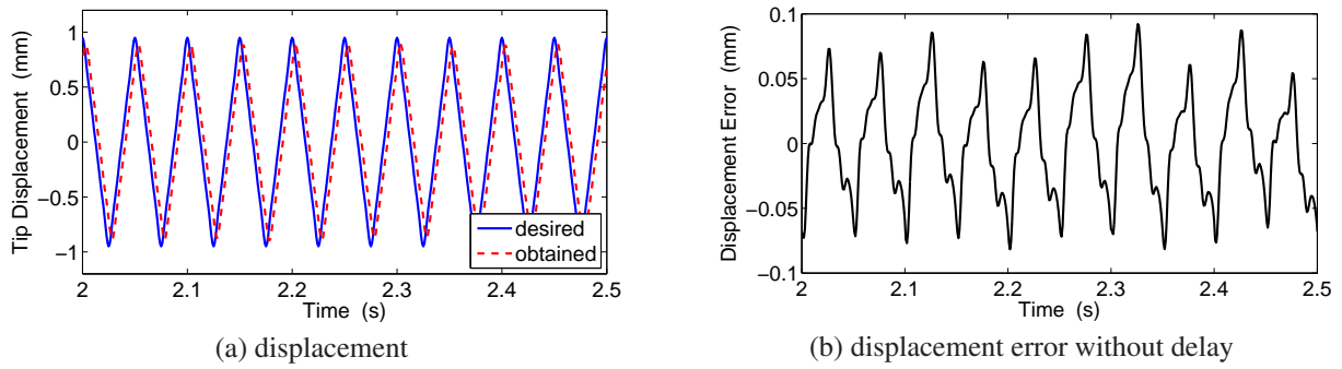
Figure 8. Experimental results of the open loop control for a desired triangular wave in the tip of the beam ( \omega_o = 20 Hz, A = 1 mm, 4 terms of the Fourier series).
