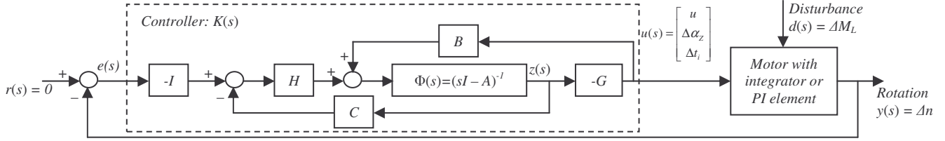
Figure 5. Compensator structure
