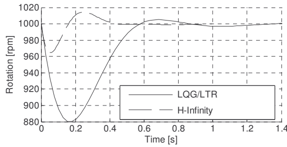
Figure 13. Step-disturbance responses for reduced and non-reduced compensator, using both methods.
