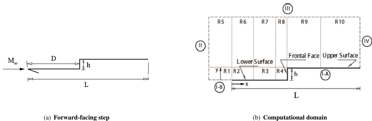
Figure 1. Drawing illustrating (a) a schematic view of the forward-facing step and (b) the computational domain.
