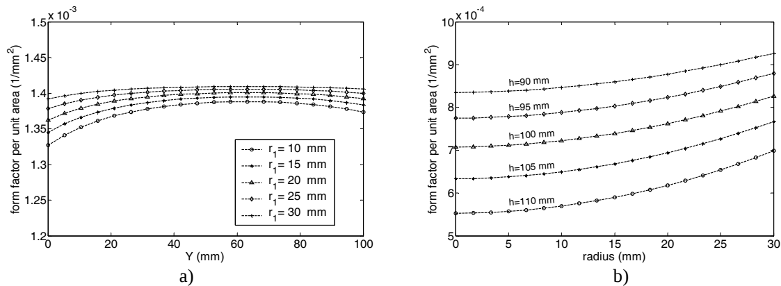
Figure 9. a) Form factor per unit area ( mm^2 ) along the side of a cylindrical sample in a cylinder calorimeter, as function of the vertical position ( y ) and radius, r_1 , of the sample. b) Form factor per unit area ( mm^2 ) along the top surface, as function of height h and radius, r_1 , of the sample.
