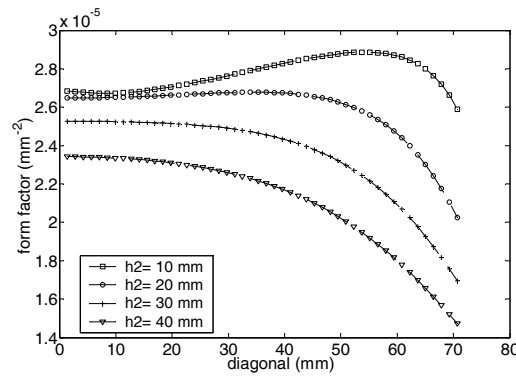
Figure 8. Form factor per unity area ( \text{mm}^2 ) along the diagonal of the exposed surface of a square slab.
