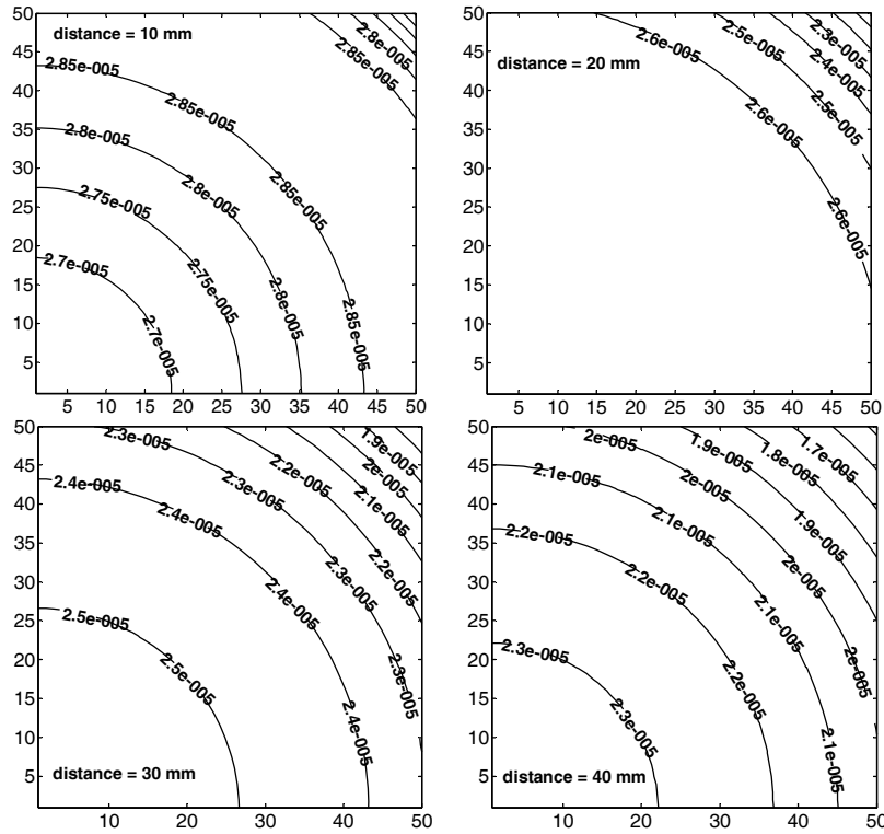
Figure 7. Effects of distance, h_2 (mm), from the sample surface to the base of a cone calorimeter, on thermal radiation distribution per unity area ( \text{mm}^2 ) of the sample surface.
