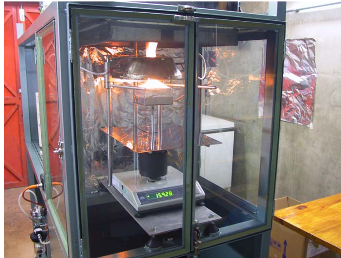
Figure 1 – Burning of pinus slabs in the cone calorimeter.
