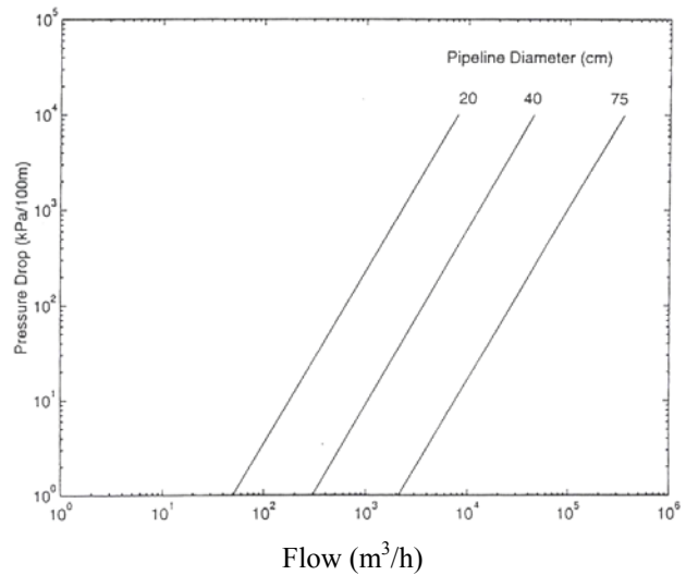
Figure 4. Oil pipeline sizing.
