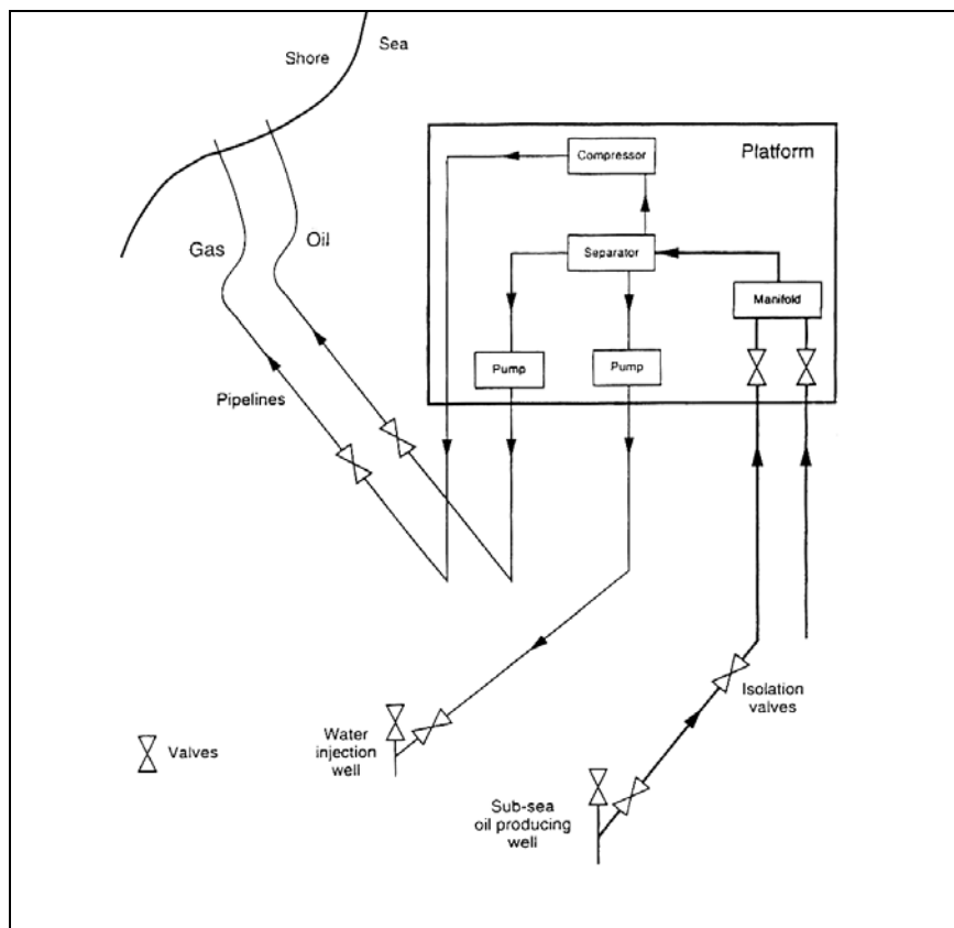
Figure 2. The field development concept with onboard separation.
