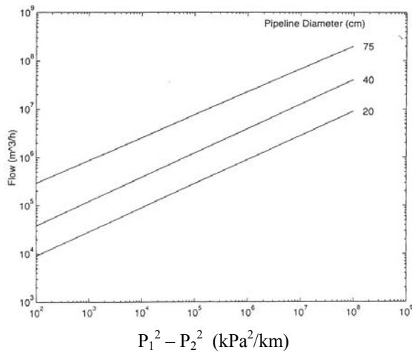
Figure 5. Gas pipeline sizing.
