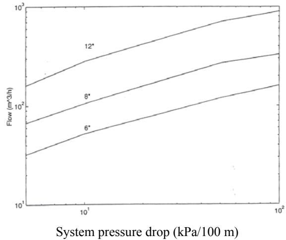
Figure 6. Typical two-phase pressure drop (well fluids with low/medium Gas-Oil Ratio) .
