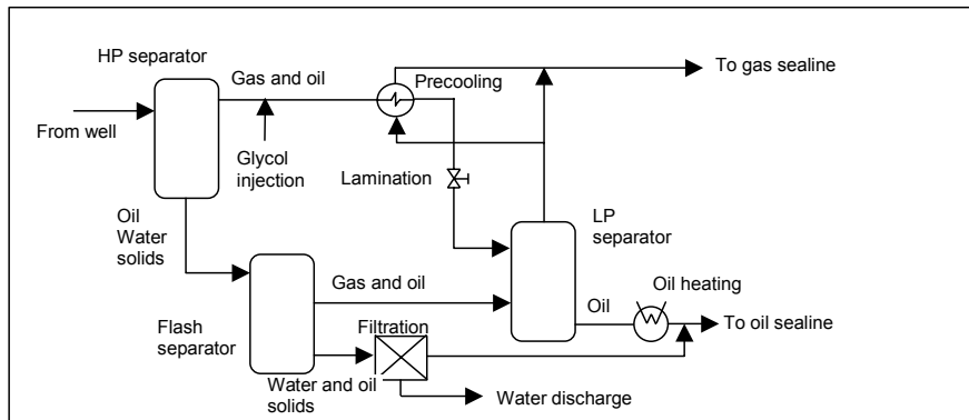
Figure 8. Scheme of a gas-oil separation plant.
