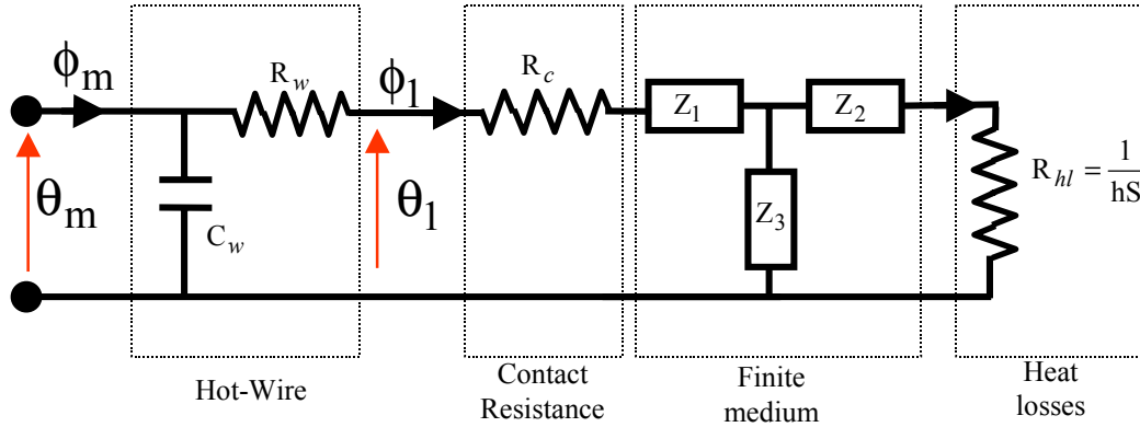
Figure 5 : Analog representation of the Hot-wire experiment.
