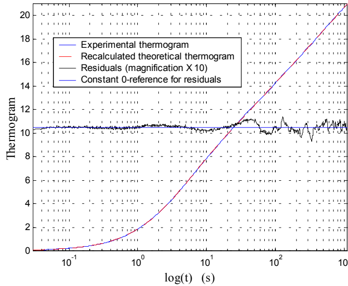
Figure 9 : Identification performed with complete model and Levenberg-Marquardt algorithm. (Number of iterations = 22, \beta_1 = 0.100, \beta_2 = 0.196, \beta_3 = t_c = 9.46, \beta_4 = 11.78, \text{ Cost} = 0.74 )
