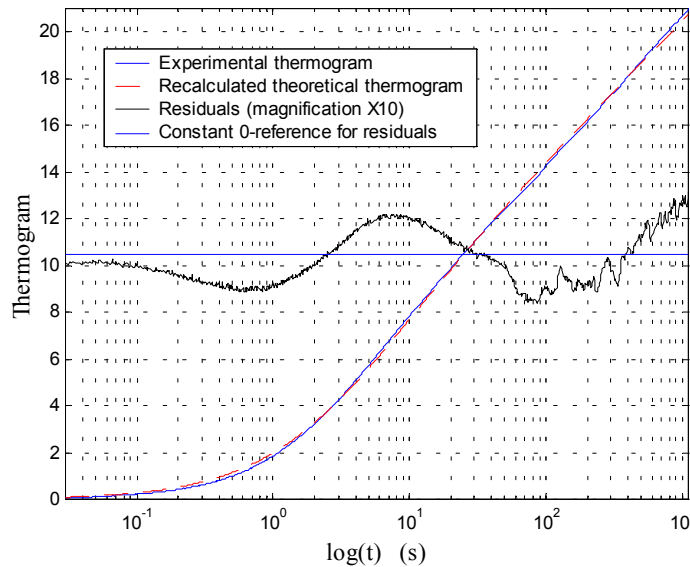
Figure 10 : Identification performed with complete model and Nelder-Mead simplex algorithm. (Number of iterations = 220, \beta_1 = 0.111, \beta_2 = 0.138, \beta_3 = t_c = 0.755, \beta_4 = 0.019, \text{ Cost} = 13.2 )
