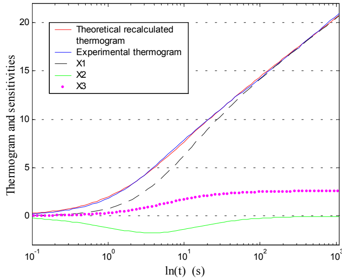
Figure 10 : Thermograms and reduced sensitivity coefficients for the case \beta_1 = 0.11, \beta_2 = 0.14, \beta_3 = t_c = 0.76 .
