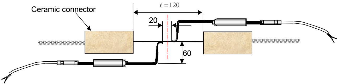
Figure 2a : Hot-wire, connections with power supplying cables and thermocouples.
