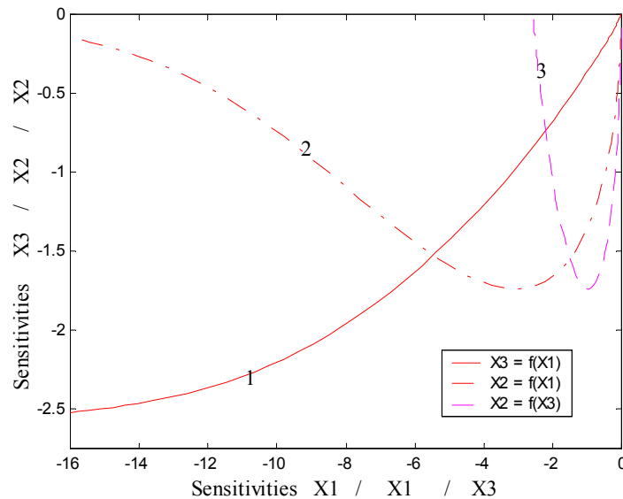
Figure 11 : Reduced sensitivity coefficients for the case \beta_1 = 0.11, \beta_2 = 0.14, \beta_3 = t_c = 0.76
