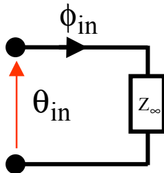
Figure 4 : Quadrupole representation of the semi-infinite layer.
