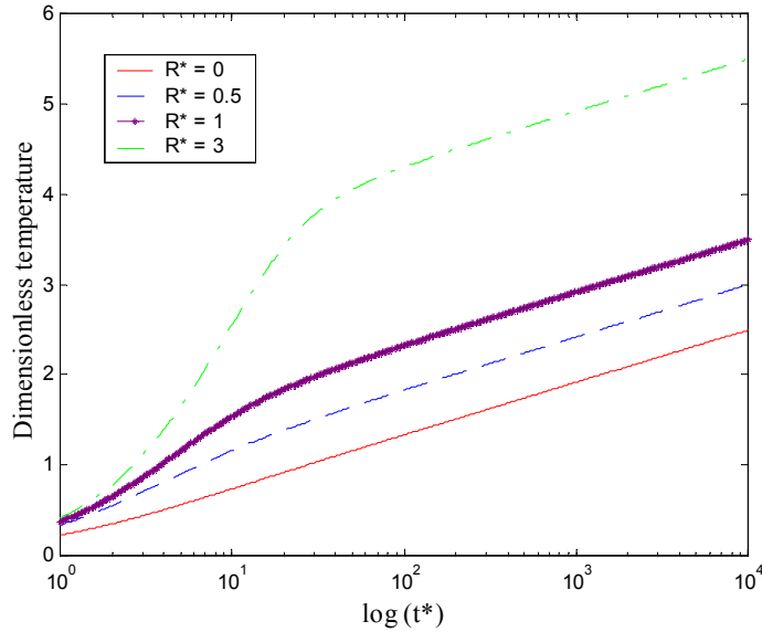
Figure 6 : Effect of the total reduced resistance ( C^* = 2.15 )
