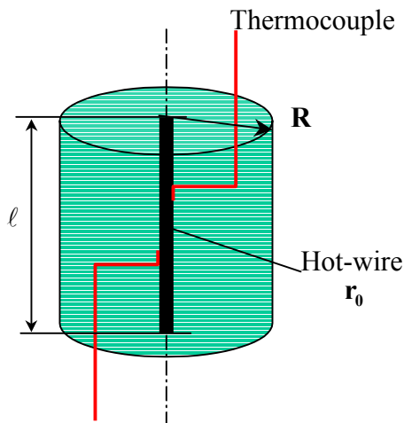
Figure 1 : Idealized theoretical model
