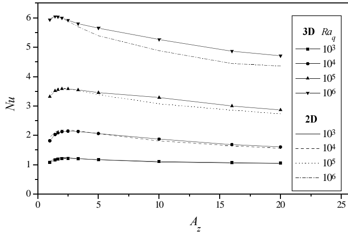
Figure 1. Average Nusselt number variation with aspect ratio A_z .
