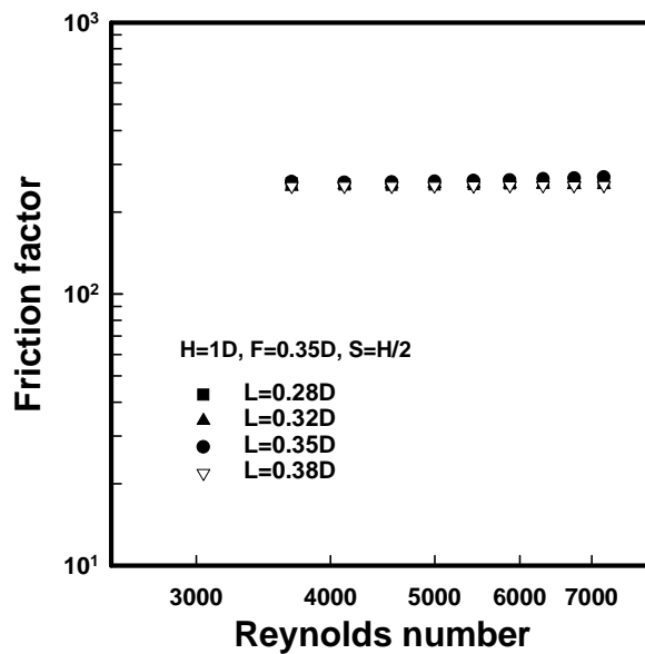
Figure 4 - The effect of the disk size on the Friction factor
