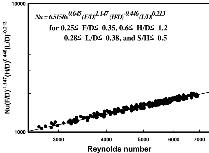
Figure 11 – A correlation for estimating the Nusselt number
