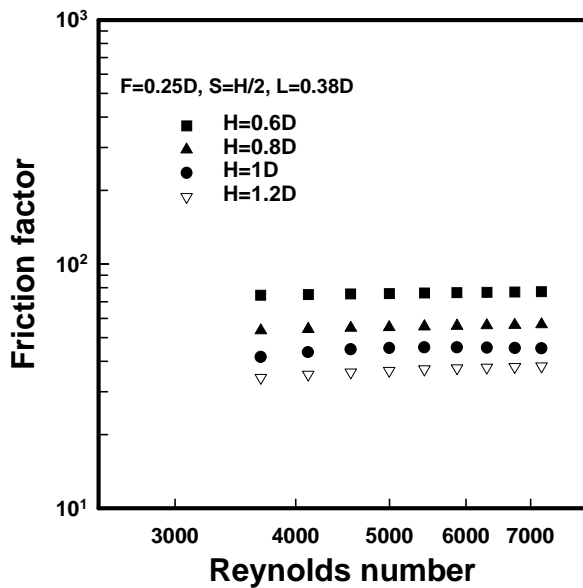
Figure 8 - The effect of the fin pitch on the Friction factor
