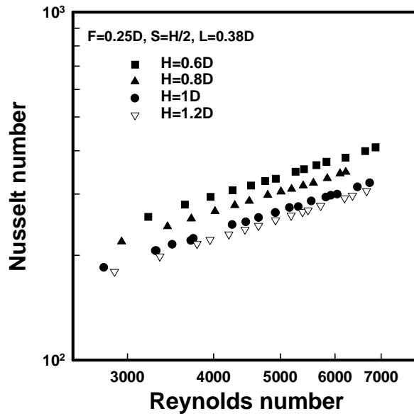
Figure 7 - The effect of the fin pitch on the Nusselt number
