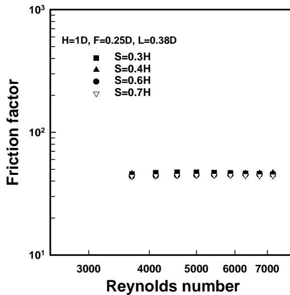
Figure 10 - The effect of the fin-disk spacing on the Friction factor
