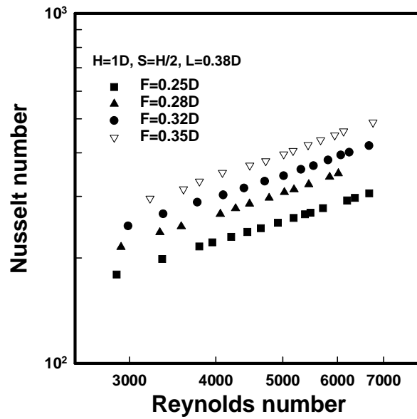
Figure 5 - The effect of the fin height on the Nusselt number
