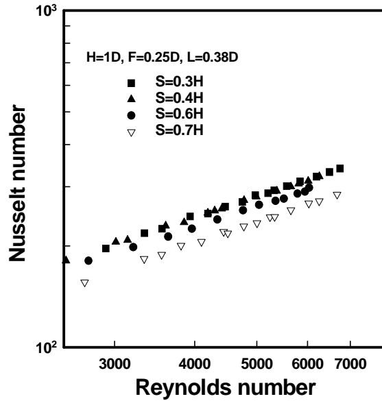
Figure 9 - The effect of the fin-disk spacing on the Nusselt number
