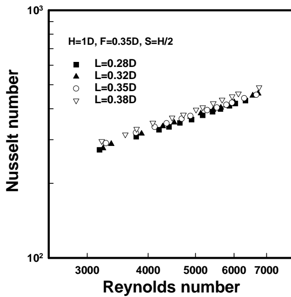
Figure 3 - The effect of the disk size on the Nusselt number
