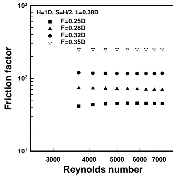
Figure 6 - The effect of the fin height on the Friction factor
