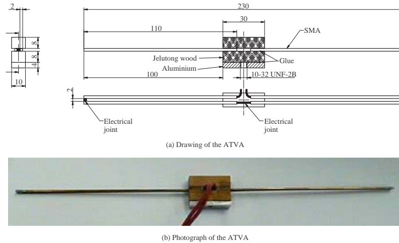
Figure 8. Prototype shape memory alloy ATVA
