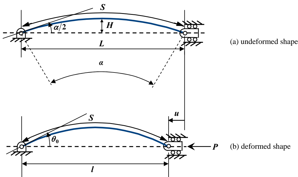
Figure 4. Curved beam loaded along its span
