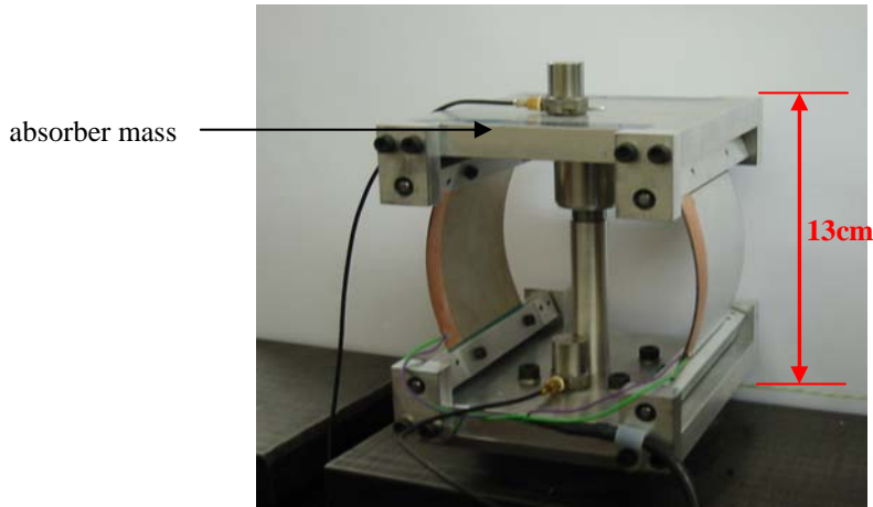
Figure 5. Prototype ATVA using curved beams as a variable stiffness element.
