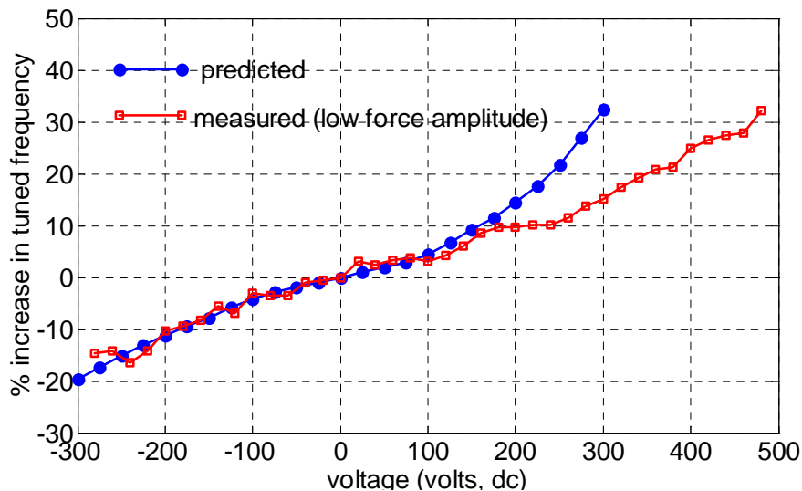
Figure 6. Tuning characteristic for the prototype ATVA shown in Figure 5
