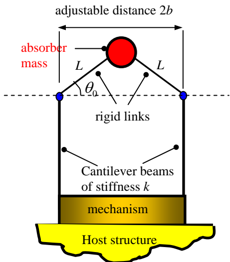
(a) diagram of the ATVA
