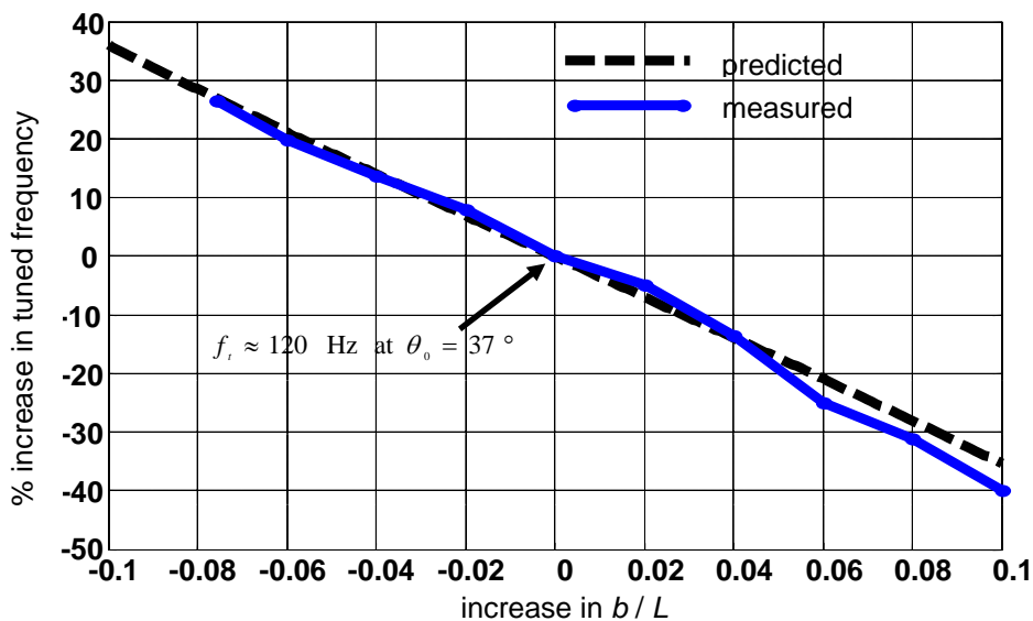
Figure 7. Tuning characteristic for the prototype ATVA shown in Figure 6
