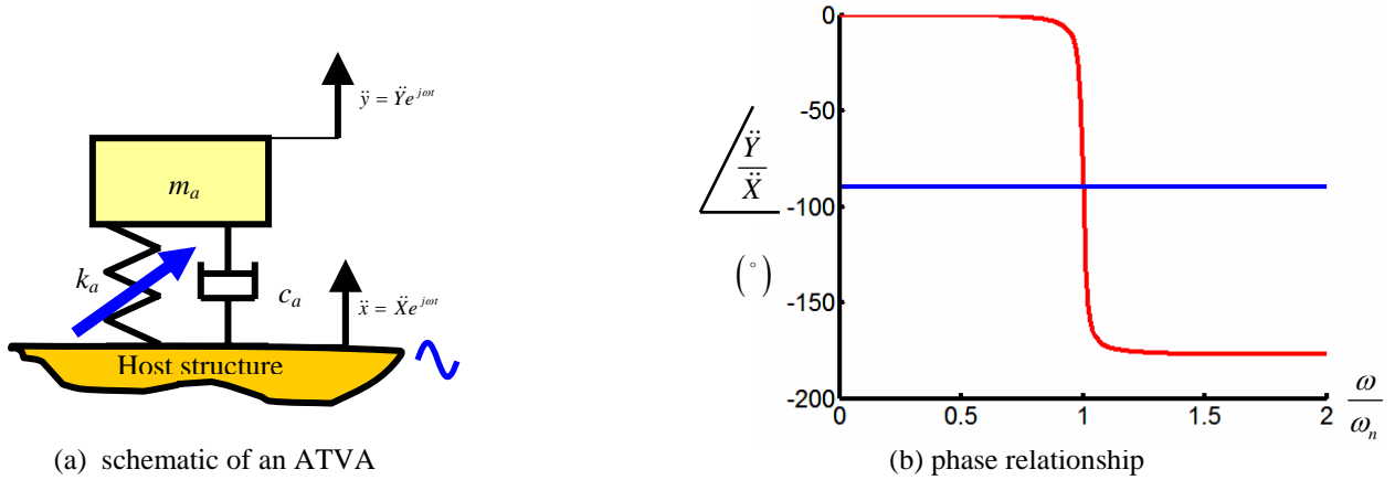
Figure 14. Schematic of an ATVA on a structure and the phase relationship between the acceleration of the host structure and the ATVA mass.
