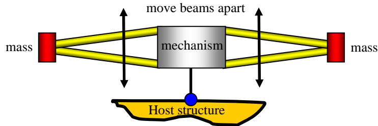
Figure 1. A beam-like vibration absorber where the stiffness is adjusted by moving the beams apart.
