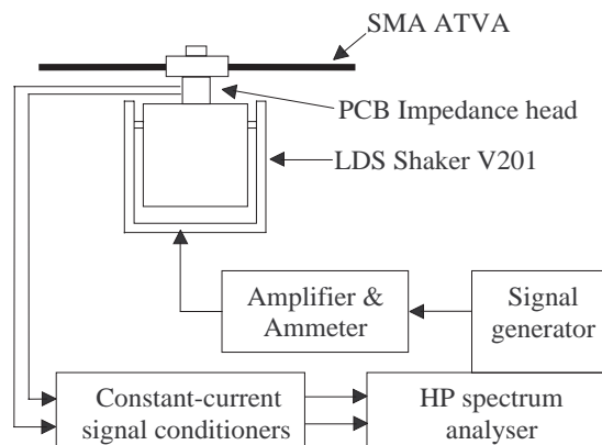
Figure 10. Experimental set-up to measure the dynamic characteristics of an SMA ATVA.
