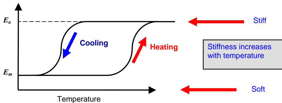
Figure 9. Young's modulus of NiTiInol SMA wire as a function of temperature. E_a and E_m denote the Young's modulus of the wire in its austenitic and martensitic states respectively. For the wire used in the prototype depicted in Figure 8, the Young's modulus changed from 40 to 59 MPa.
