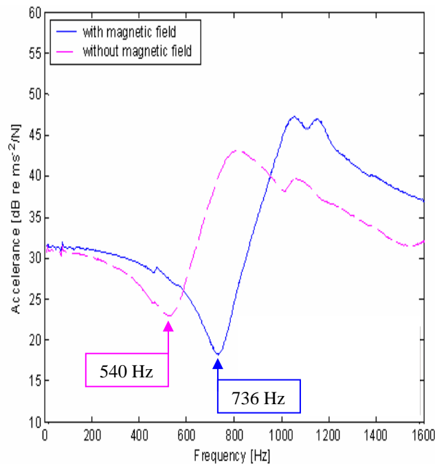
Figure 13. Measured accelerance of the tunable fluid-filled beam ATVA
