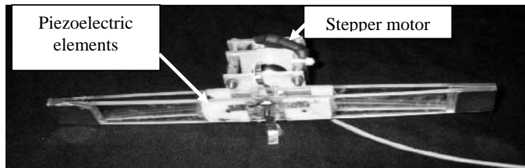
Figure 2. Experimental beam-like ATVA.
