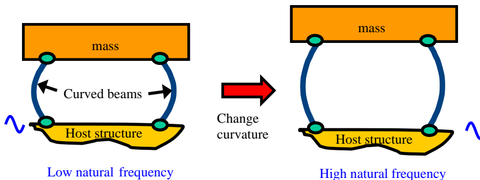
Figure 3. ATVA with stiffness element formed from parallel curved beams. As the beams straighten, the natural frequency increases
