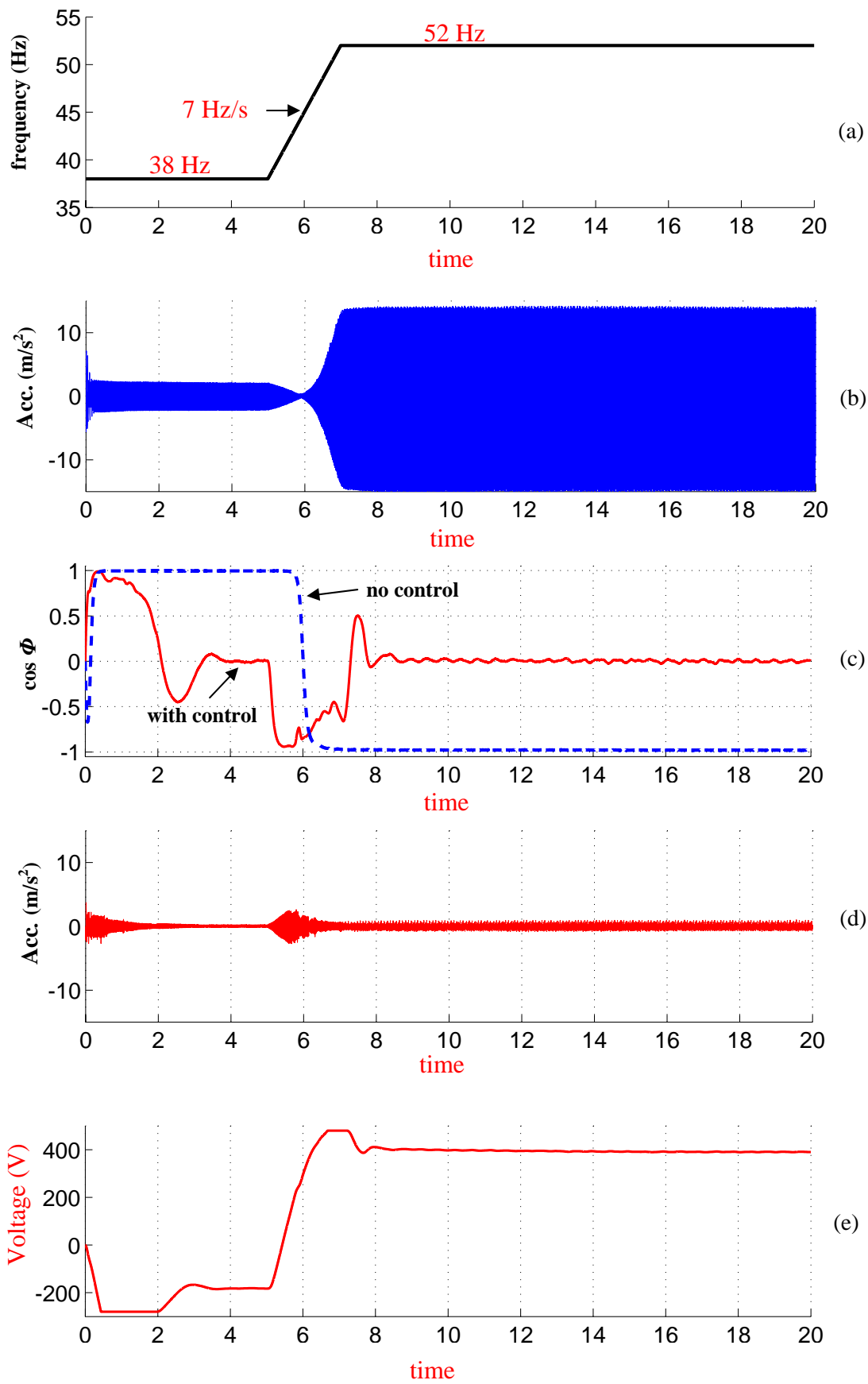
Figure 15. Experimental results for variable frequency harmonic excitation. (a) frequency variation; (b) vibration \ddot{x} without control, piezo-actuators at 0 V; (c) cosine of \phi ; (d) controlled vibration \ddot{x} ; (e) variation of controlled voltage applied to piezo-actuators; for control results P = 4 \times 10^{-2} , D = 8 \times 10^{-3} .
