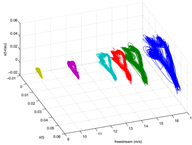
Figure 9: Evolution with respect to the freestream velocity of reconstructed state spaces for free turntable cases.
