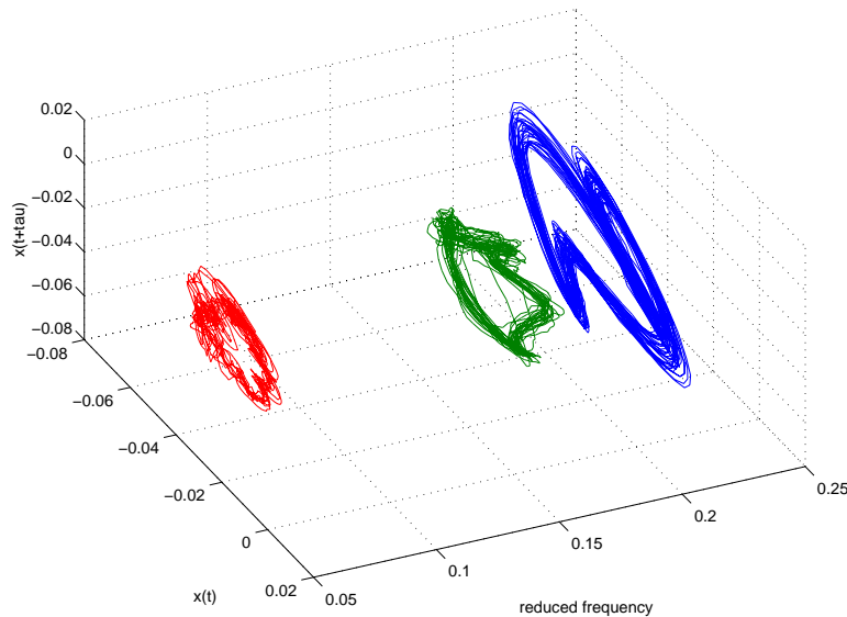
Figure 6: Reconstructed state spaces for bending measurements with reduced frequency variation (cases 3 to 5 from Tab. 1).
