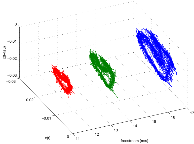
Figure 7: Reconstructed state spaces of torsional measurements with freestream velocity variation (cases 2, 4 and 6 from Tab. 2).
