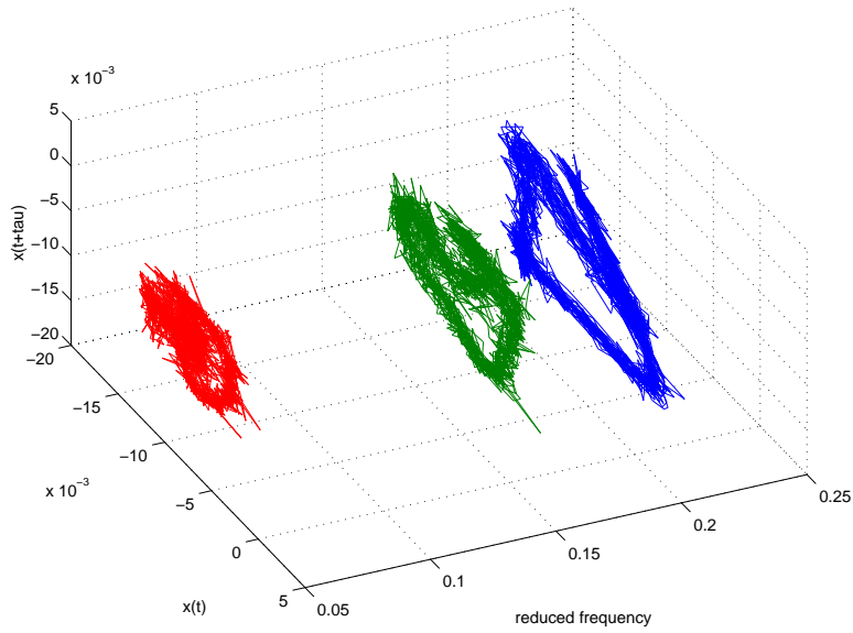
Figure 8: Reconstructed state spaces for torsional measurements with reduced frequency variation (cases 3 to 5 from Tab. 2).
