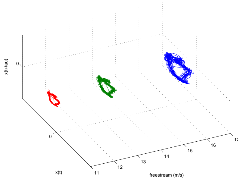
Figure 5: Reconstructed state spaces of bending measurements with freestream velocity variation (cases 2, 4 and 6 from Tab. 1).
