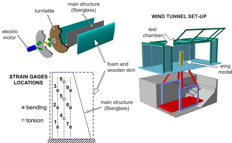
Figure 1: Experimental set-up and strain gages locations.
