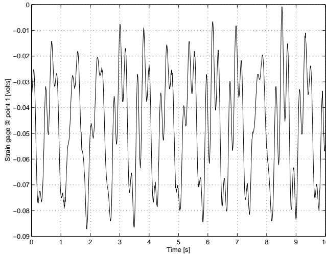
Figure 2: Aeroelastic response time history (oscillatory case).
