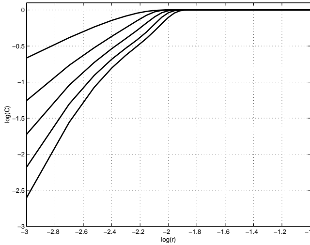
Figure 4: Determination of the embedding (or attractor) dimension ( d ).
