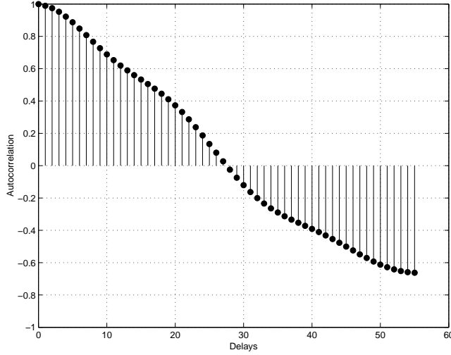
Figure 3: Autocorrelation function and the time delay ( T ) determination.
