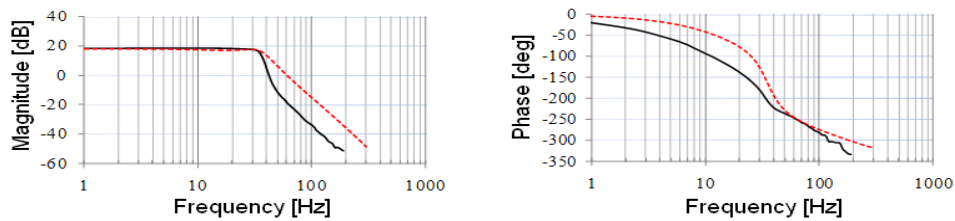
Figure 7. Valve pressure-to-voltage Bode diagram: experiments (solid) and simulation (dashed)
