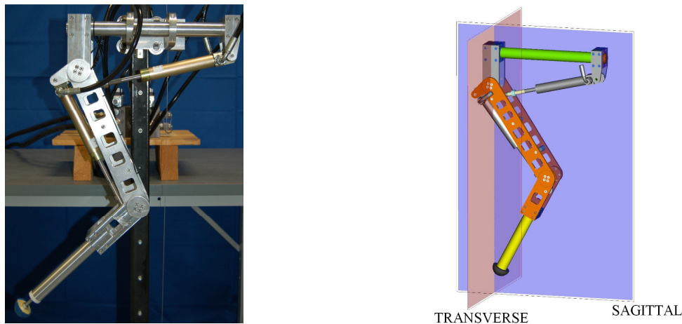
Figure 1. Picture of the HyQ leg prototype (version 1) with its hydraulic actuation and the definition of the sagittal (blue) and transverse (red) planes
