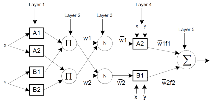
Figure 1. ANFIS Structure.
