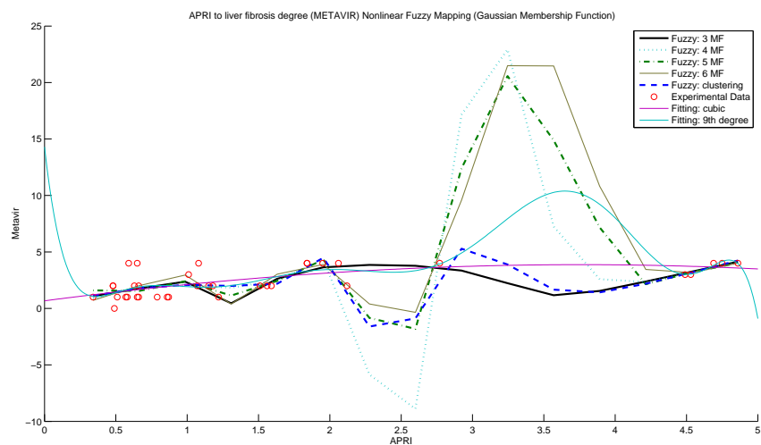
(c) Gaussian Membership Function with 3, 4, 5, and 6 Membership Function.
