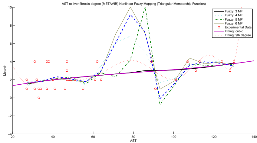
(a) Triangular Membership Function with 3, 4, 5, and 6 Membership Function.
