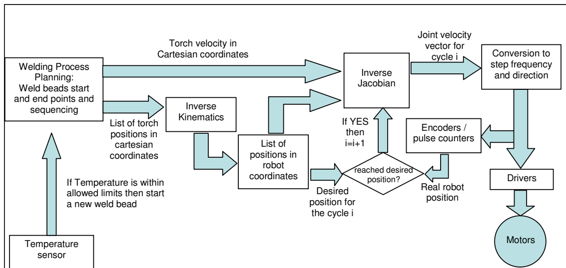
Figure 4 – Robot control scheme
