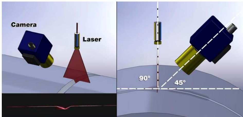
Figure 5: Image triangulation scheme
