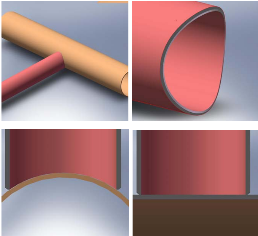
Figure 12: T junction, very common on hot tapping procedures, with complex trajectories, and variable junction to be welded, with almost flat groove at 0° and 180°.
