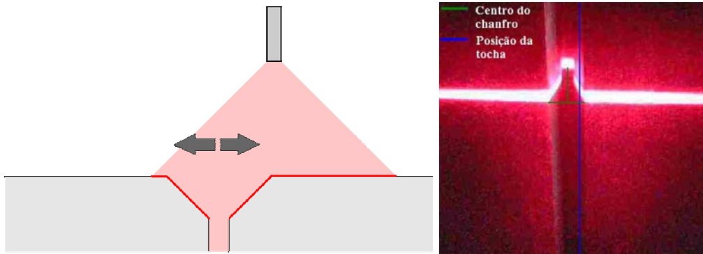
Figure 7: Trajectory deviations detection.
