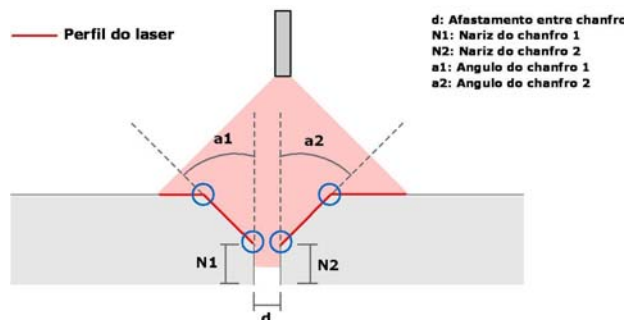
Fig. 6: Features extracted from the groove.
