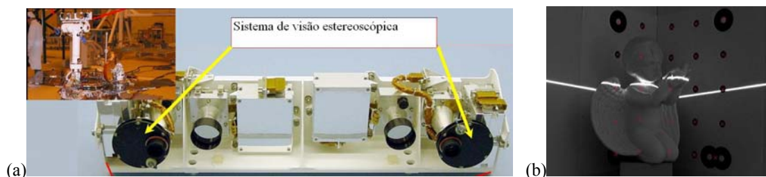
Figure 2: Stereoscopic vision system of Mars exploration rovers (NASA/JPL) (a), and structured vision system (David-Laserscan) (b).
