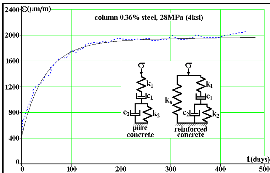
Figure 11: Strain history \varepsilon(t) for a f'_c = 28MPa reinforced concrete column with steel area fraction f_{a_s} = 0.36\% , loaded by a fixed force that induces an initial strain \varepsilon_0 = 400\mu m/m ( k_1 = 24.87GPa , c_1 = 70TPa \cdot day , k_2 = 6GPa and c_2 = 300GPa \cdot day .)
