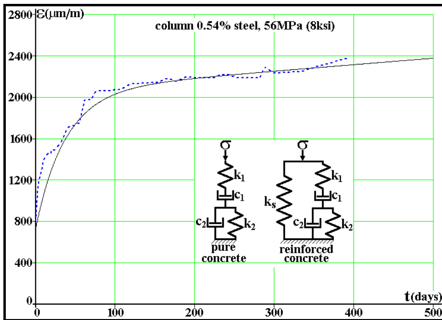
Figure 9: Strain history \varepsilon(t) for a f'_c = 56\text{MPa} reinforced concrete column with steel area fraction f_{a_s} = 0.54\% , loaded by a force that causes an initial strain \varepsilon_0 = 800\mu\text{m/m} (curve generated using k_1 = 24.87\text{GPa} , c_1 = 80\text{TPa}\cdot\text{day} , k_2 = 6.5\text{GPa} and c_2 = 340\text{GPa}\cdot\text{day} .)
