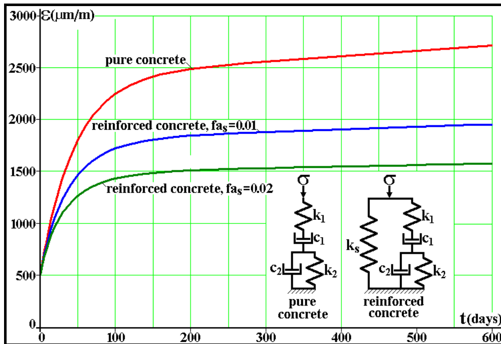
Figure 7: Strain histories \varepsilon(t) estimated by equation (10) for a pure concrete and for two steel reinforced concrete columns with steel area fractions f_{a_s} = 1\% and f_{a_s} = 2\% , when they are loaded by a fixed force that causes an initial strain \varepsilon_0 = 500\mu\text{m}/\text{m} . The concrete is modeled as a linear viscoelastic Burgers' material with constant parameters k_1 = 21\text{GPa} , c_1 = 1.814\text{TPa}\cdot\text{s} , k_2 = 5.8\text{GPa} e c_2 = 21.6\text{GPa}\cdot\text{s} , whereas the steel reinforcement is modeled as a Hookean material with k_s = 200\text{GPa} .
