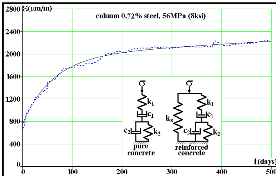
Figure 8: Total (elastic plus creep) strain history \varepsilon(t) estimated by equation (10) for a reinforced concrete column with f'_c = 56\text{MPa} and steel area fraction f_{a_s} = 0.72\% , loaded by a fixed force that induces an initial (elastic) strain \varepsilon_0 = 800\mu\text{m/m} (curve generated by using the fitted viscoelastic parameters k_1 = 37.54\text{GPa} , c_1 = 40\text{TPa}\cdot\text{day} , k_2 = 19\text{GPa} and c_2 = 1.2\text{TPa}\cdot\text{day} .)
