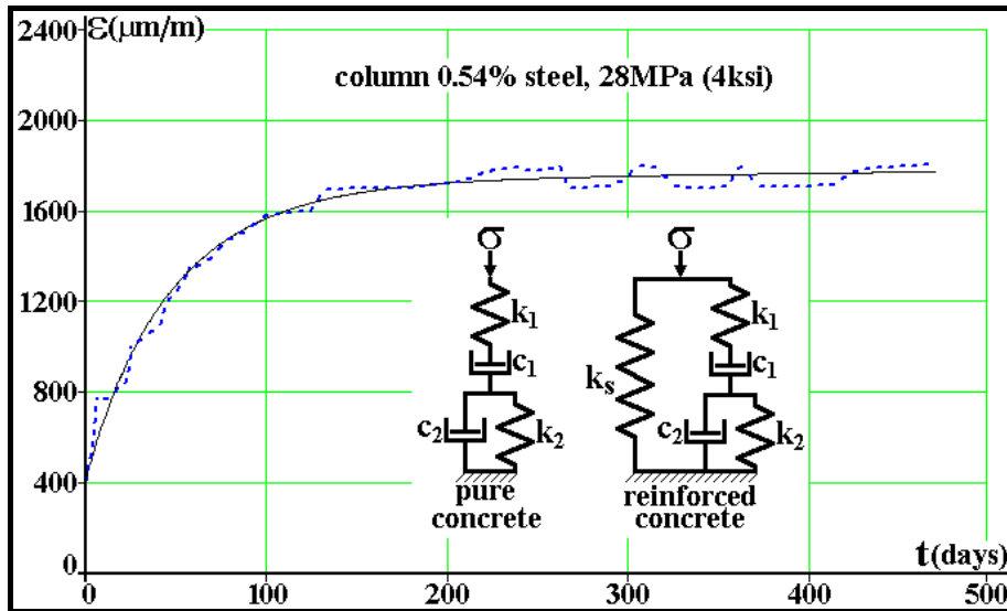
Figure 10: Strain history \varepsilon(t) for a f'_c = 28MPa reinforced concrete column with steel area fraction f_{a_s} = 0.54\% , loaded by a fixed force that induces an initial strain \varepsilon_0 = 400\mu m/m ( k_1 = 24.87GPa , c_1 = 80TPa \cdot day , k_2 = 6.5GPa and c_2 = 340GPa \cdot day .)
