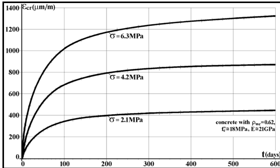
Figure 4: Time variation of creep strains under compressive stresses (plotted as positives for convenience) for a concrete with compressive strength f'_c = 18 \text{ MPa} , Young's modulus E_{c28} \cong 1.36(\rho_c^3 \cdot f'_c)^{0.5} \cong 21 \text{ GPa} (both measured, as usual, 28 days after casting), water/cement ratio \rho_{wc} = 0.62 , and density \rho_c \cong 2.3 .
