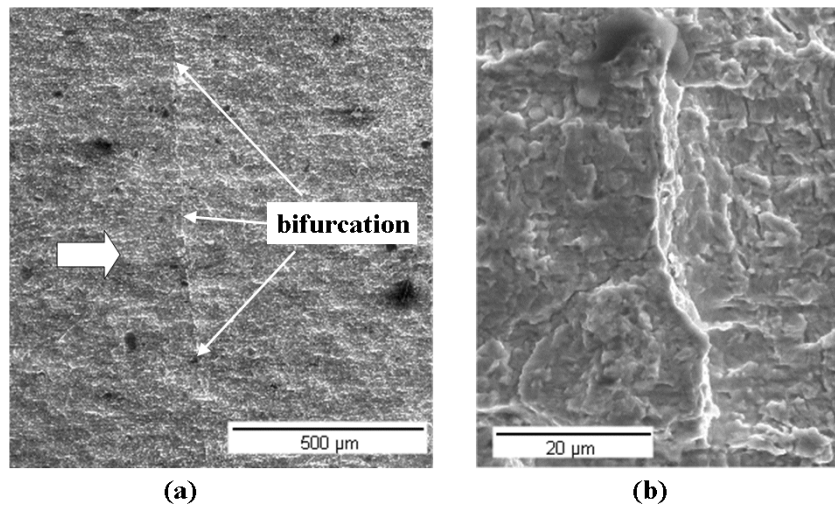
Fig. 8. Scanning electron micrographs of fracture surfaces (test II): (a) bifurcation front through the specimen thickness, and (b) detailed view indicating different height levels.
