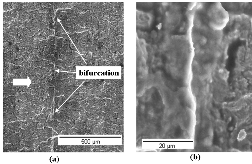
Fig. 7. Scanning electron micrographs of fracture surfaces (test I): (a) bifurcation front through the specimen thickness, and (b) detailed view indicating different height levels.
