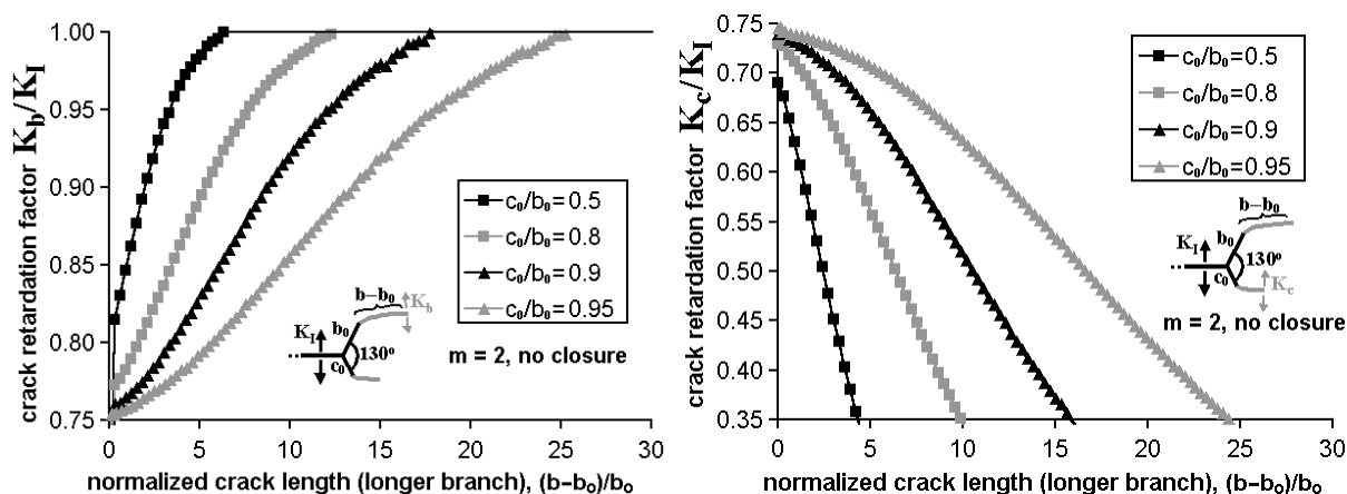
Fig. 2. Normalized equivalent SIF for the (a) longer and (b) shorter branch of a bifurcated crack during its propagation ( 2\theta = 130^\circ , m = 2 , K_{PR} = 0 ).
