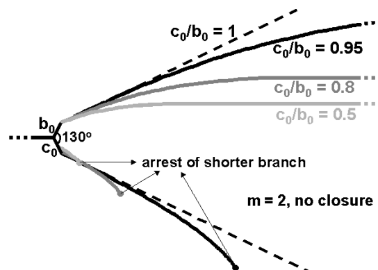
Fig. 1. Bifurcated crack paths for several c_0/b_0 ratios ( K_{PR} = 0 ).
