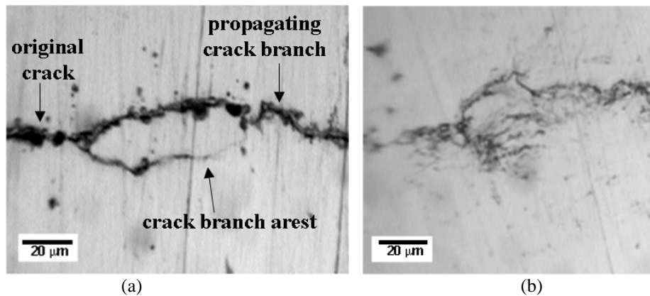
Fig. 4. Crack bifurcation experiments on SAE 4340 steel: (a) test I, (b) test II.
