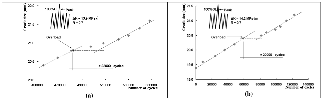
Fig. 5. Fatigue crack growth retardation after a 100% overload with R = 0.7 : (a) test I and (b) test II.
