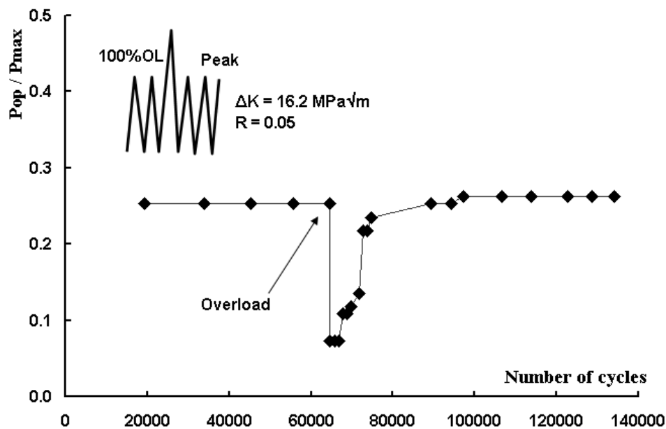
Fig. 11. Opening load measurements, before and after the overload (test IV).
