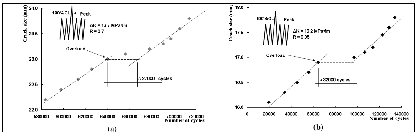
Fig. 6. Fatigue crack growth retardation after a 100 % overload: (a) R = 0.7 , test III; (b) R = 0.05 , test IV.
