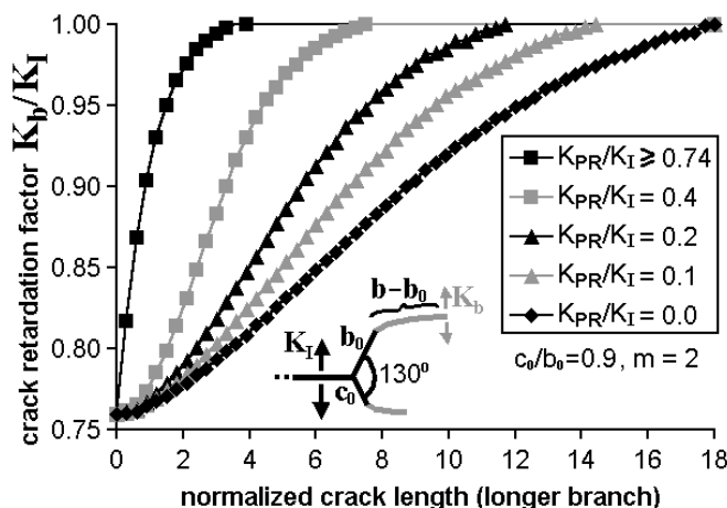
Fig. 3. Normalized SIF of the longer branch during its propagation as a function of the normalized length (b-b_0)/b_0 for several K_{PR} levels ( c_0/b_0 = 0.9 , m = 2 ).
