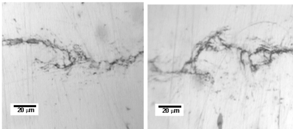
Fig. 10. Crack bifurcation experiments on SAE 4340 steel (test IV): (a) front face of specimen (b) back face of specimen.
