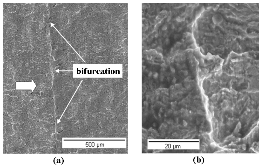
Fig. 9. Scanning electron micrographs of fracture surfaces (test III): (a) bifurcation front through the specimen thickness, and (b) detailed view indicating different height levels.
