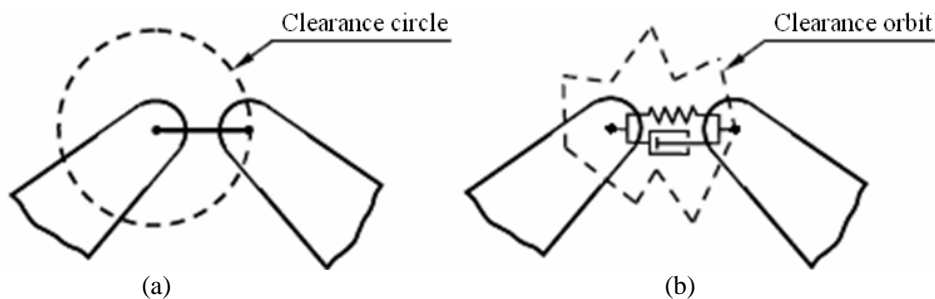
Figure 2. Examples of models for revolute joints with clearance: (a) massless link model; (b) spring-damper model (Fernandes, 2005).
