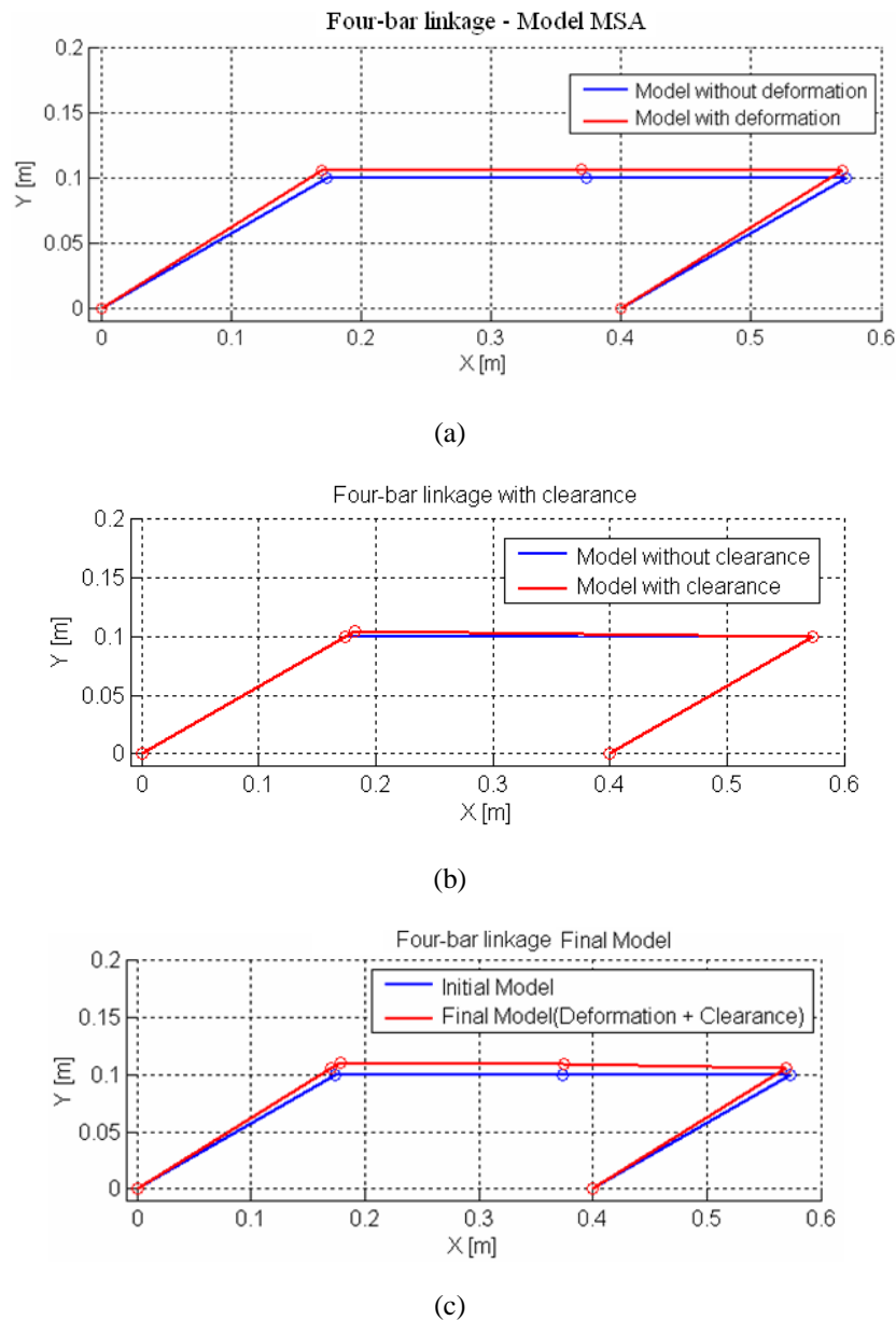
Figure 7. Configurations of the four-bar linkage. (a) structure behavior due to compliant displacement; (b) structure behavior due to the effects of joint clearance; (c) final configuration superposing both displacements.
