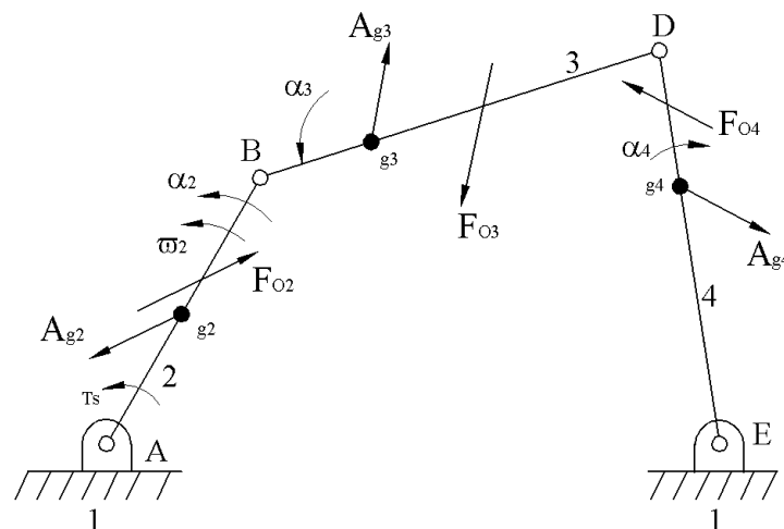
Figure 4. Inertia forces, accelerations and velocities of the four-bar linkage (Erdman and Sandor, 1991).
