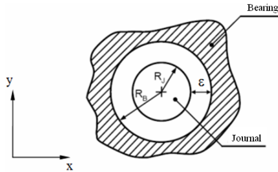
Figure 1. Revolute joint with clearance.
