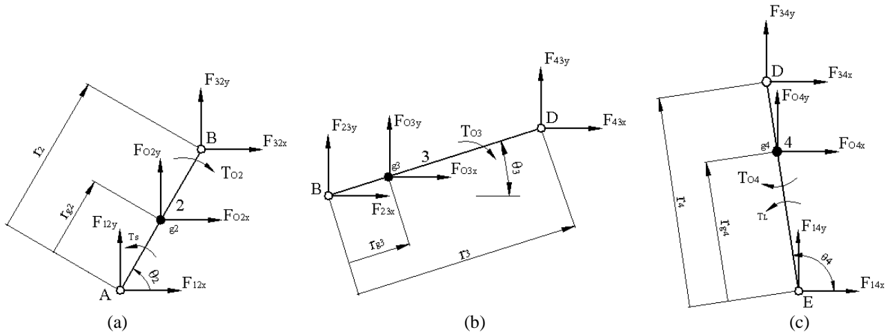
Figure 5. (a), (b) and (c) show free-body diagrams of links used for the kinetostatic equilibrium (Erdman and Sandor, 1991).
