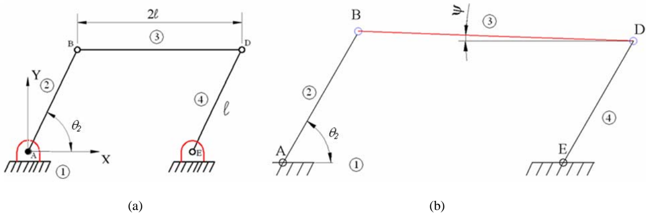
Figure 6. (a) Symmetric four-bar linkage; (b) Angular motion \psi of link ③.
