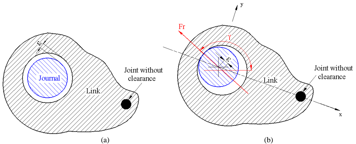
Figure 3. (a) Model of clearance; (b) Reaction force.
