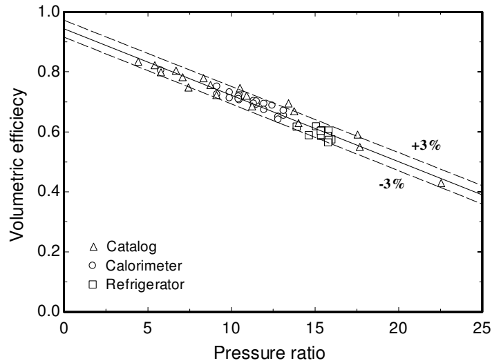
Figure 3. Correlation between the volumetric efficiency and the pressure ratio
