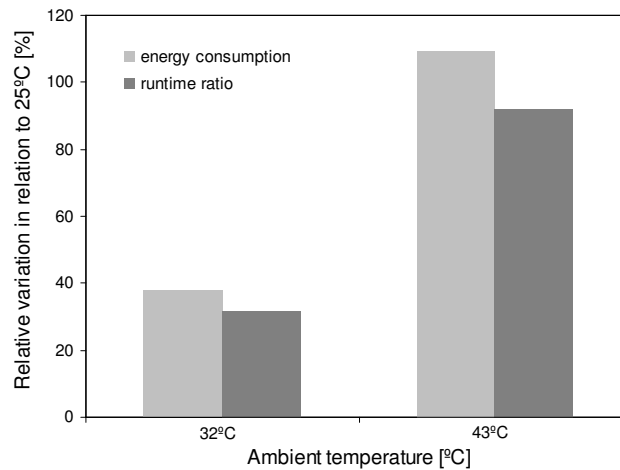
Figure 6. Variation of the energy consumption and runtime ratio with ambient temperature
