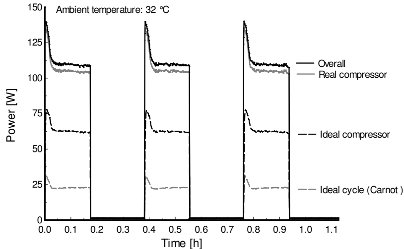
Figure 8. Variation of the power consumption with time
