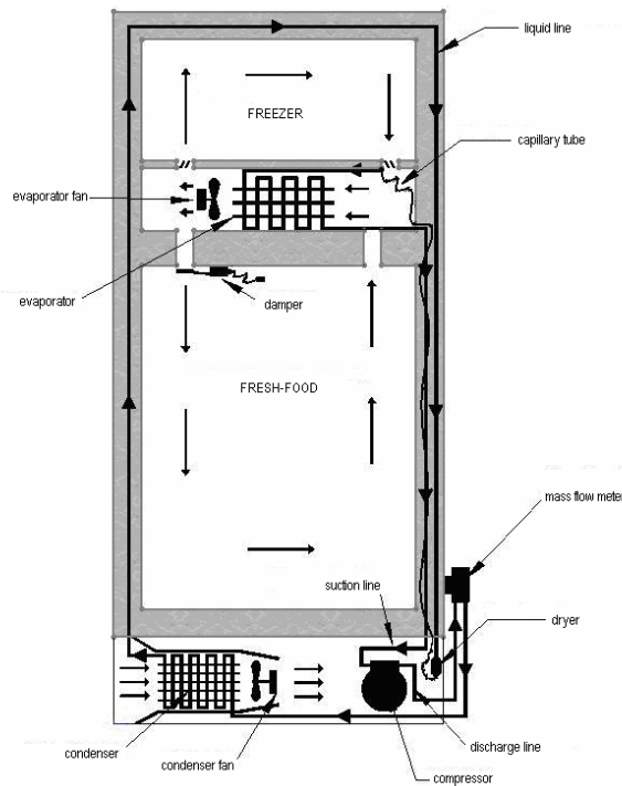
Figure 1. Schematic representation of the household refrigerator tested
