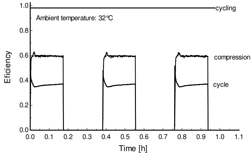
Figure 10. Variation of the system efficiencies with time
