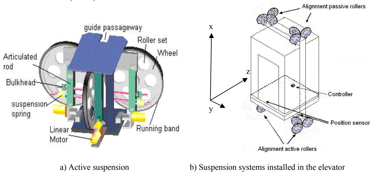
Figure 1: Suspension system
