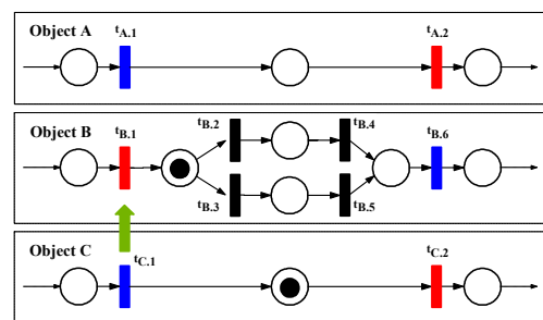
(d) Object C calls a method provided by Object B through the fusion of transitions t_{C,1} and t_{B,1}
