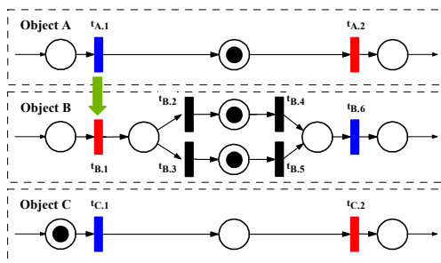
(a) Object B is executing a method required by Object A, through the fusion of transitions t_{B,1} and t_{A,1} , while Object C is waiting for the availability of Object B
