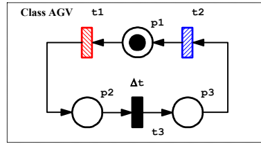
Figure 4. A simplified model of an AGV.
