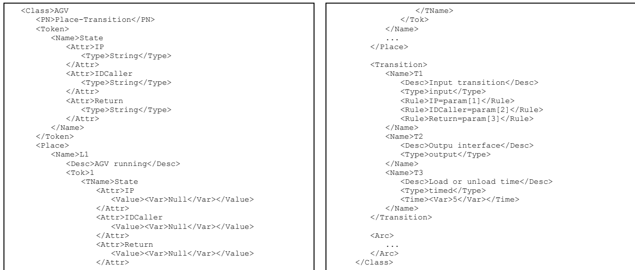
Figure 5. AGV model textual description.
