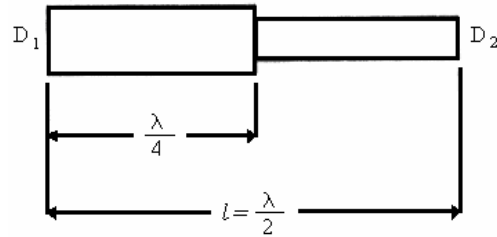
Figure 3. Half-wave Stepped acoustic amplifier.
