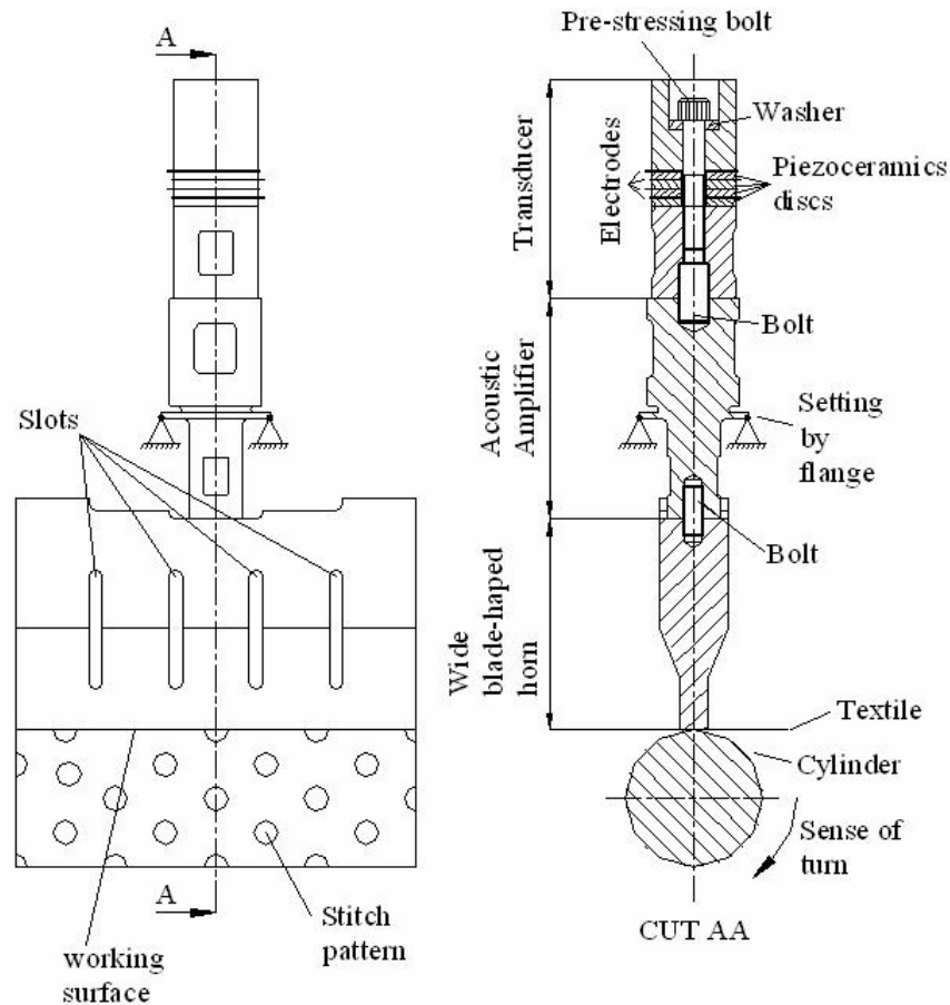
Figure 1. Schematic representation of the assembly of ultrasonic cutting and welding of thermoplastic textile.
