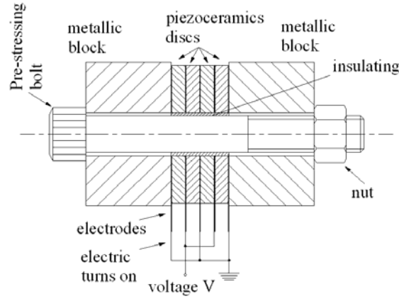
Figure 2. Sandwich piezoelectric transducer in cut view.
