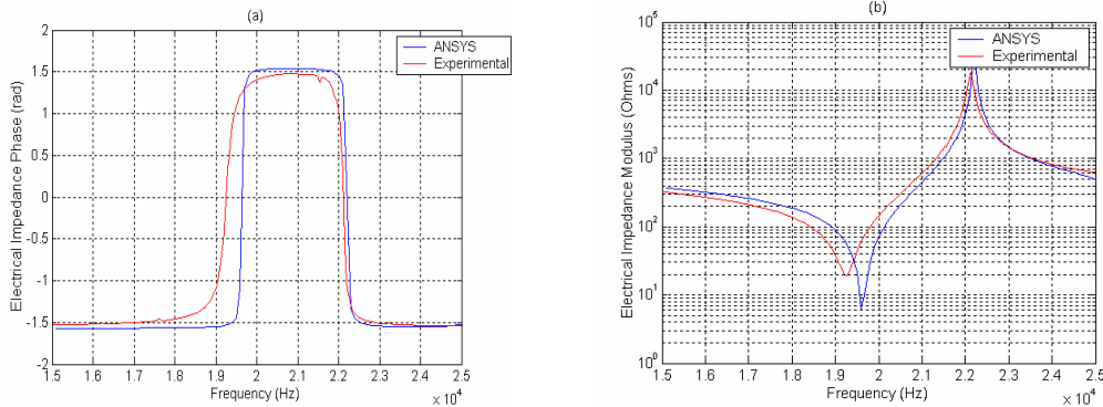
Figure 8. (a) Electrical impedance phase curves obtained for the transducer assembled with eight piezoceramic discs. (b) Electrical impedance modulus curves obtained for the transducer assembled with eight piezoceramic discs.
