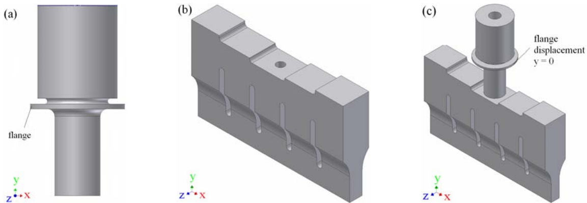
Figure 6. Models (a) acoustic amplifier. (b) wide blade-shaped horn. (c) acoustic amplifier-wide horn assembly.
