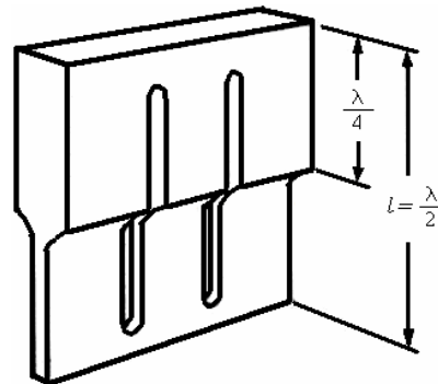
Figure 4. Wide blade-shaped horn.
