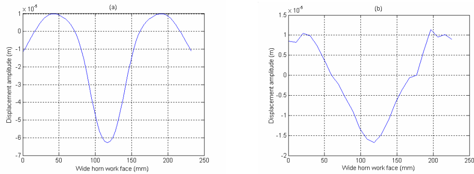
Figure 11. (a) Topography of the displacement at work face wide horn obtained numerically. (b) Topography of the displacement at work face wide horn obtained experimentally.
