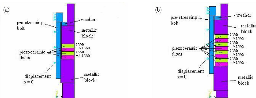
Figure 5. Model of the high power piezoelectric transducer (a) with four piezoceramic discs. (b) with eight piezoceramic discs.
