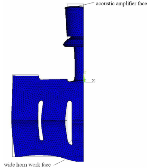
Figure 9. Vibration mode of the acoustic amplifier-wide horn assembly.
