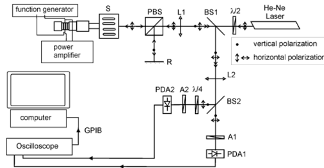
Figure 10. Experimental setup of Michelson-type quadrature interferometer.
