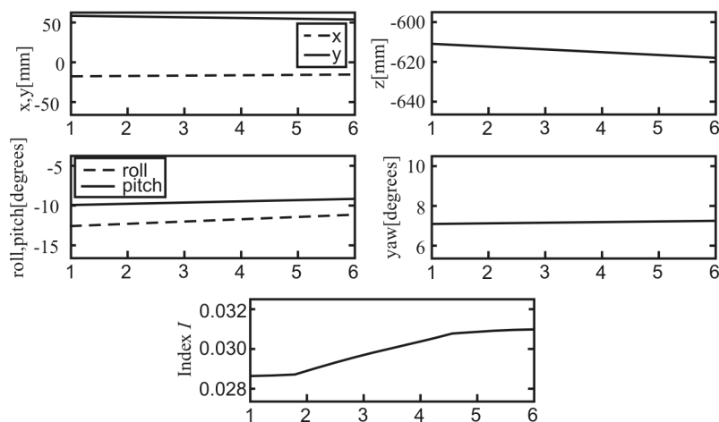
Figure 3. The automatic movement of the tool to escape the singularity (all x axes show time[s])
