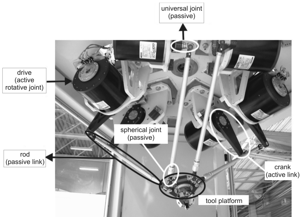
Figure 1. The Hexa parallel robot
