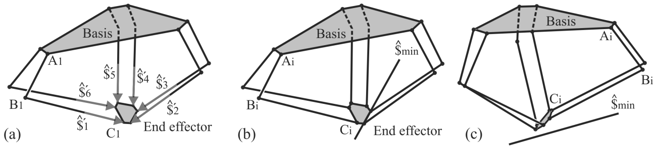
Figure 2. (a) The wrenches acting upon the moving platform. (b) and (c) Two direct singularities
