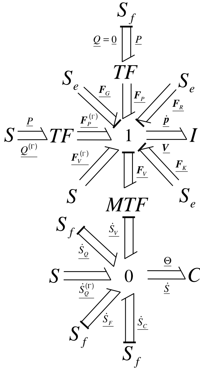
Figure 8. System Bond Graph for an incompressible fluid.
