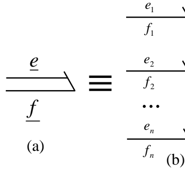
Figure 4. Multibond with nodal vector of scalar variables (a), equivalent to n single bonds (b).
