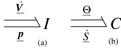
Figure 1. Inertial (a) and capacitive (b) fields, representing kinetic and internal energy storage for an incompressible fluid.
