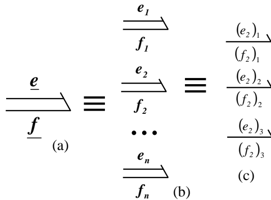
Figure 3. Multibond with nodal vector of vector variables for a three dimensional problem (a), equivalent to n multibonds of vector variables (b), each one of these equivalent to three single bonds (c).
