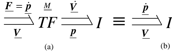
Figure 2. Multibond transformer connected to the inertial port (a), and equivalent inertia field for incompressible flow (b).
