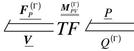
Figure 7. Multibond transformer representing the superficial pressure force.
