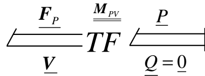
Figure 6. Multibond transformer representing the integral incompressibility constraint.
