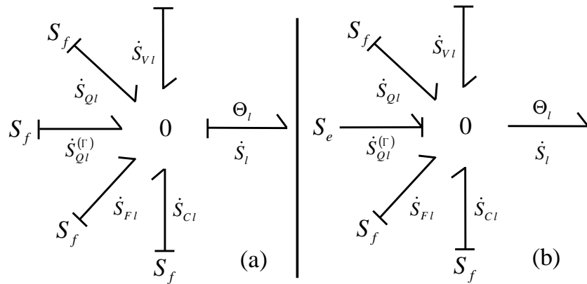
Figure 10. Causality extensions at a C -field port, integral (a) and derivative (b).
