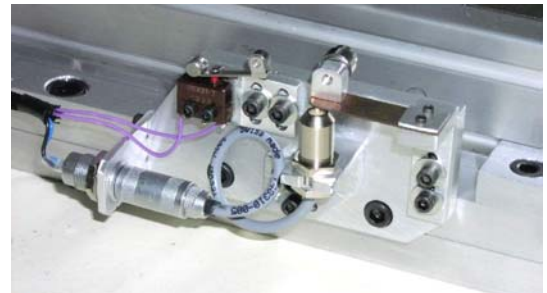
Figure 10 - Fiducial system.
