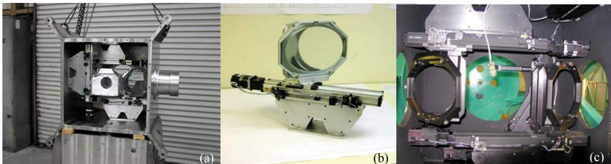
Figure 4 - SOAR IR-ISM steering mechanisms.
