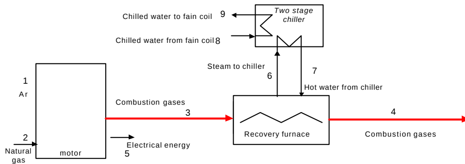
Figure 1 – Simplified diagram of the 1st configuration proposed for the shopping center under study.
