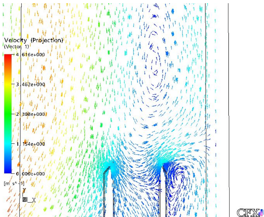
Figure 5. Zoom in the counterflow configuration.
