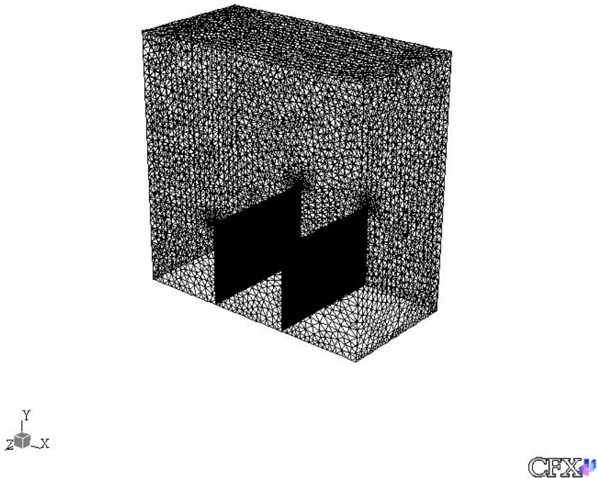
Figure 1. The grid of half box in numerical experiment
