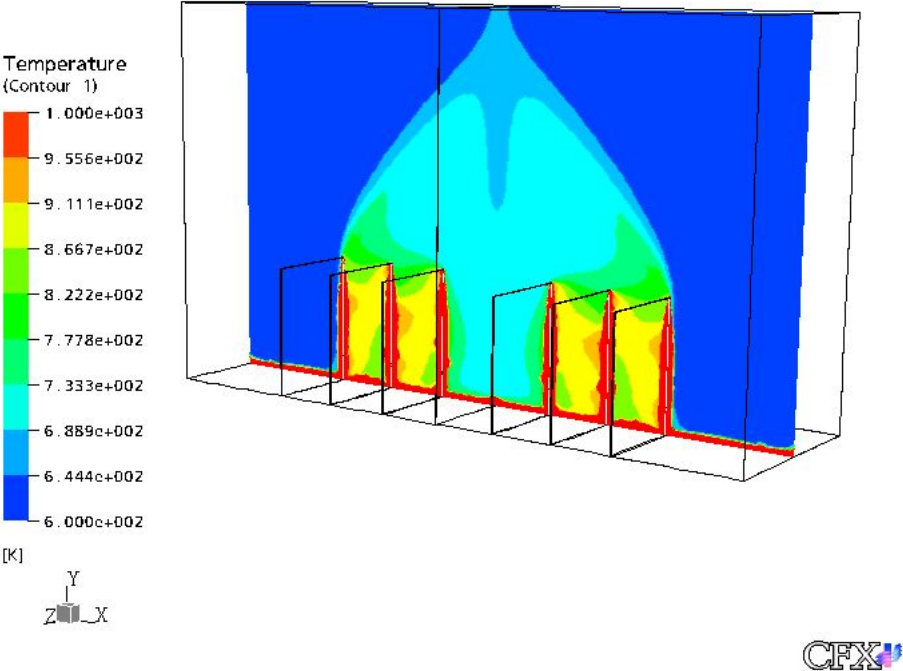
Figure 3. Temperature field
