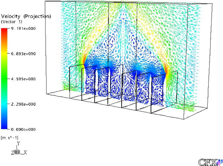
Figure 2. Velocity field
