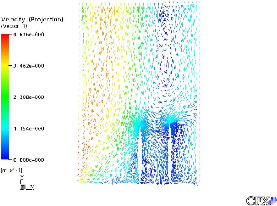
Figure 4. Flow field generated by two vertical plates.
