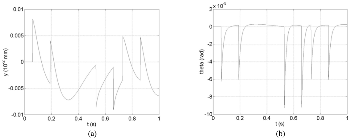
Figure 12. Material: ABS, damped, L_1=2L/5 , L_2=3L/5 , tube without surface waviness (a) y[10^{-2} \text{ mm}] \times t[\text{s}] ; (b) \theta[\text{rad}] \times t[\text{s}] .
