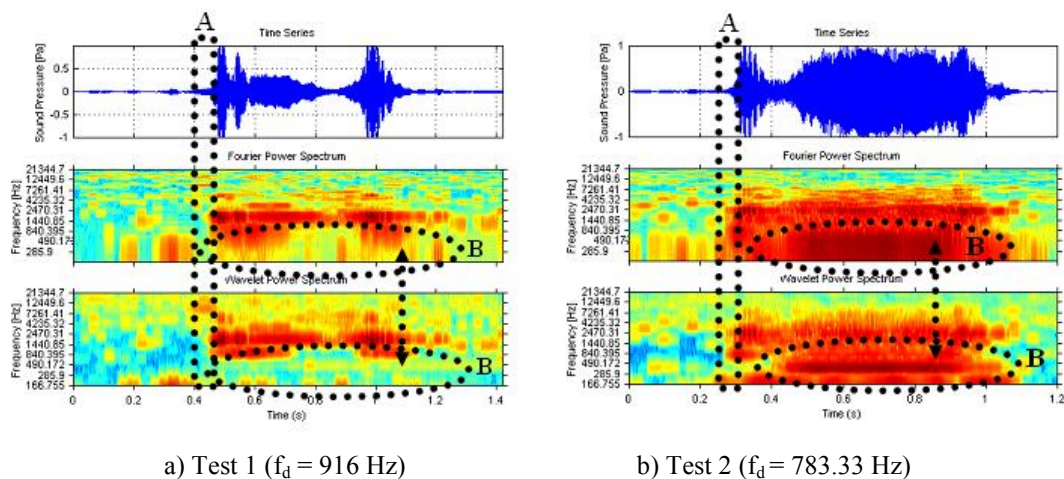
Figure 4. Fourier and Wavelet power spectrum of stable conditions signals
