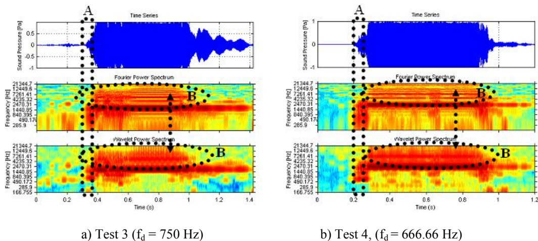
Figure 5. Fourier and Wavelet power spectrum of unstable conditions signals
