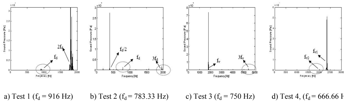
Figure 3. Frequency spectrum record for stable (a,b) and unstable (c,d) conditions
