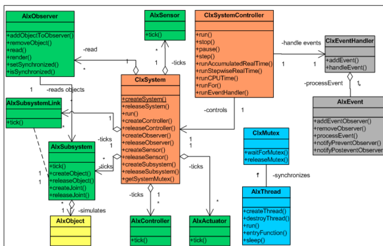
Figure 1. UML Diagram of the most important classes
