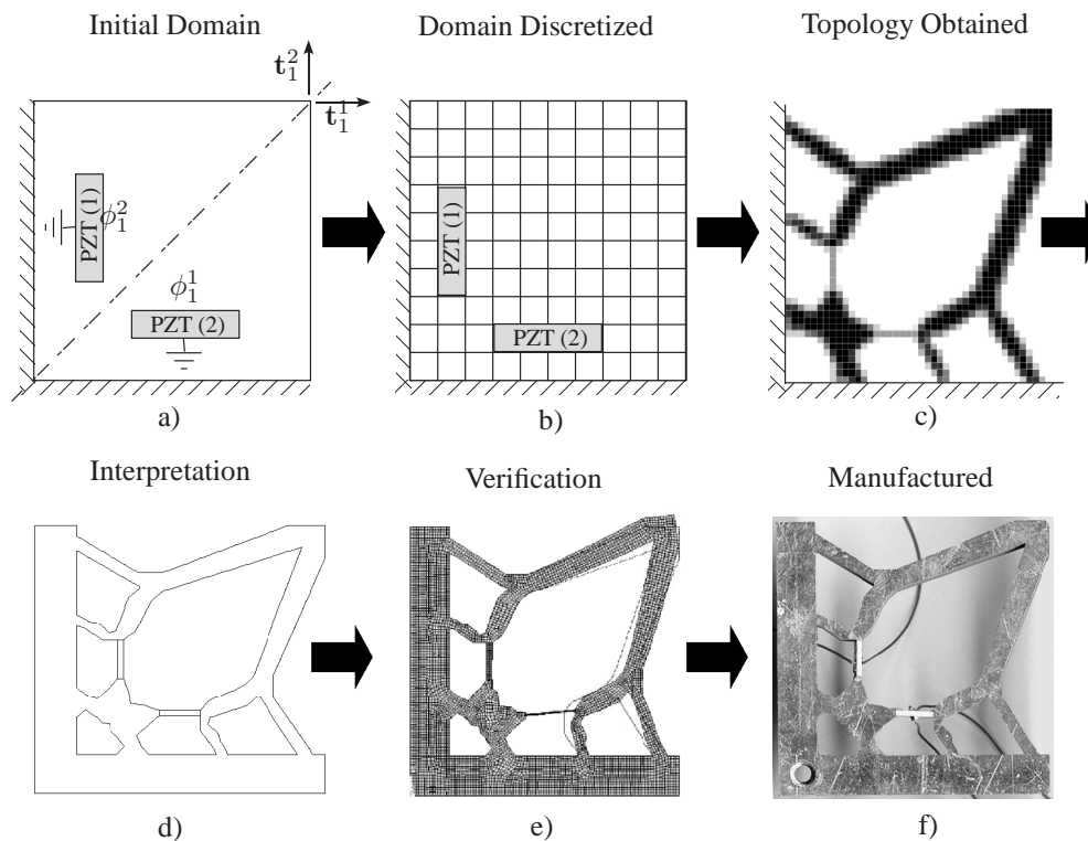
Figure 3. Topology optimization procedure for designing piezoelectric mechanisms. \Delta u is the desired output displacement.
