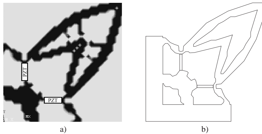
Figure 7. a) Topology optimization result for actuator XY08; b) Corresponding interpretation (CAD design).
