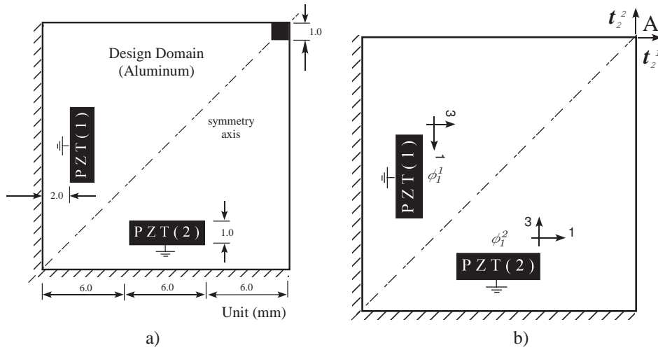
Figure 4. a) Initial Design domain; b) Design specifications for XY nanopositioners.
