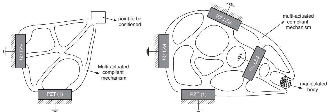
Figure 1. Concept of a multi-actuated flextensional piezoelectric devices. a) XY nanopositioner; b) Piezoceramics are responsible for XY displacements, rotation, and open/close movement of jaw.
