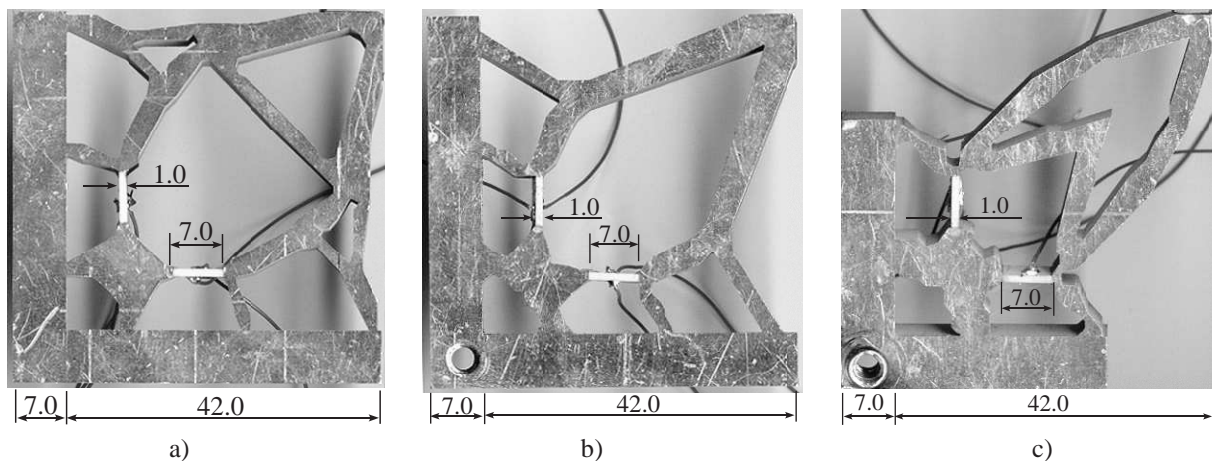
Figure 2. XY nanopositioner prototypes (unit mm); a) XY05b, b) XY05, and c) XY08.
