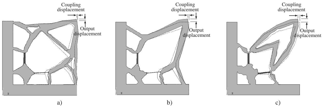
Figure 8. Displacement of XY nanopositioner obtained by FEM. a) XY05b, b) XY05, and c) XY08.
