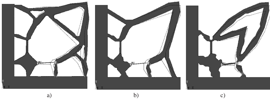
Figure 9. Von Mises stress distribution of XY nanopositioner obtained by FEM. a) XY05b, b) XY05, and c) XY08.
