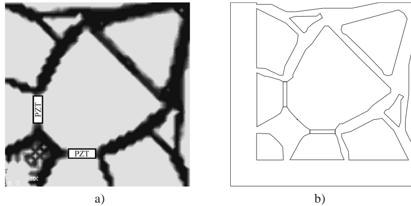
Figure 5. a) Topology optimization result for actuator XY05b; b) Corresponding interpretation (CAD design).
