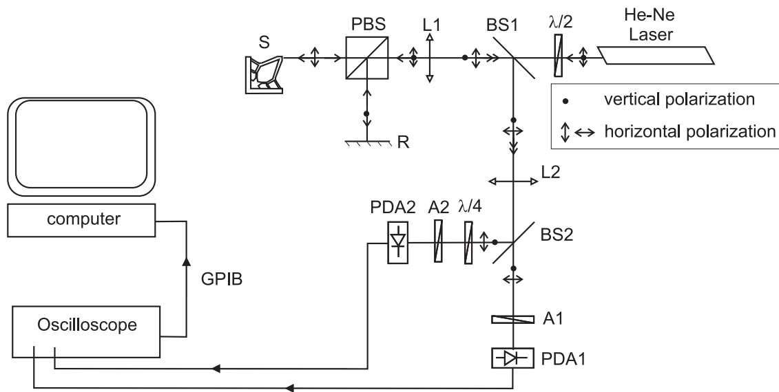
Figure 10. Experimental setup of Michelson-type quadrature interferometer. L1, L2 - convergent lens; BS1, BS2 - beam splitter; PBS - polarizing beam splitter; R - reference mirror; S - sample; \lambda/2 - half-wave plate; \lambda/4 - quarter-wave plate at 45^\circ ; A1, A2 - polarizing at 45^\circ ; PDA1, PDA2 - amplified photo-diode, GPIB - communication protocol.
