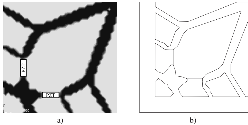
Figure 6. a) Topology optimization result for actuator XY05; b) Corresponding interpretation (CAD design).
