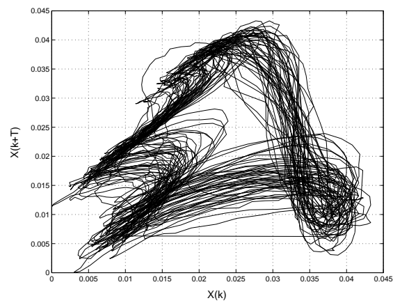
Figure 4. Reconstructed space state for case 5 without low pass filtering.
