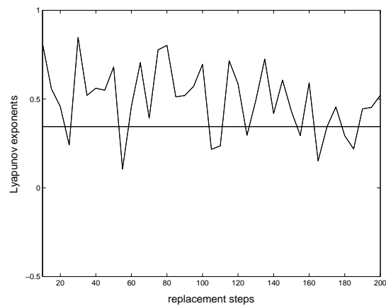
Figure 8. Evolution of the Lyapunov exponent with respect to replacement steps.
