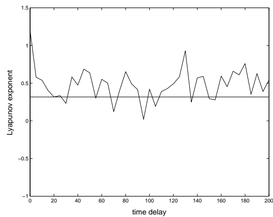
Figure 7. Evolution of the Lyapunov exponent with respect to time delay with low pass filtering.
