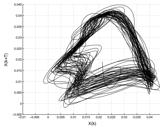
Figure 5. Reconstructed space state for case 5 with low pass filtering.
