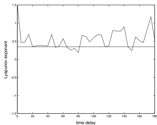
Figure 6. Evolution of the Lyapunov exponent with respect to time delay.
