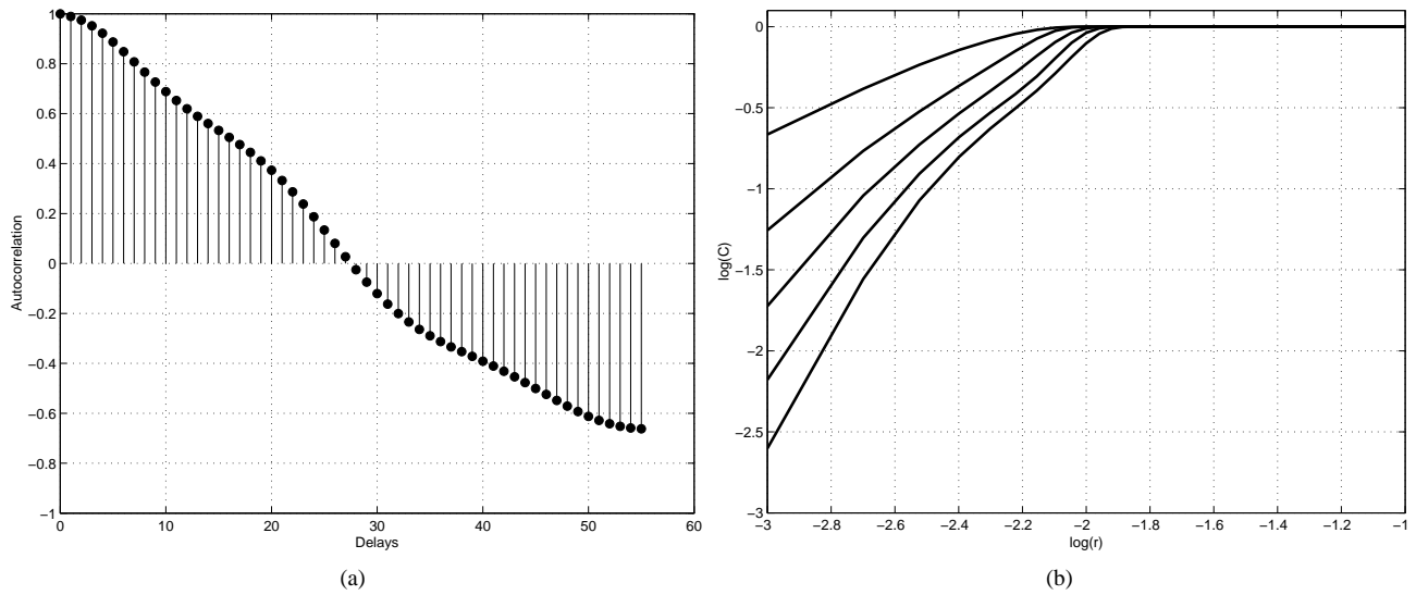
Figure 2. (a)Time delay determination. (b)Embedding dimension determination.
