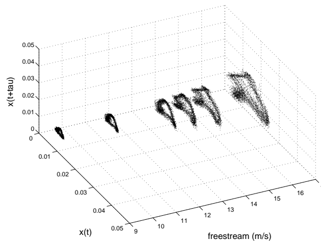
Figure 3. Evolution with respect to the freestream velocity of reconstructed state spaces for free turntable cases.
