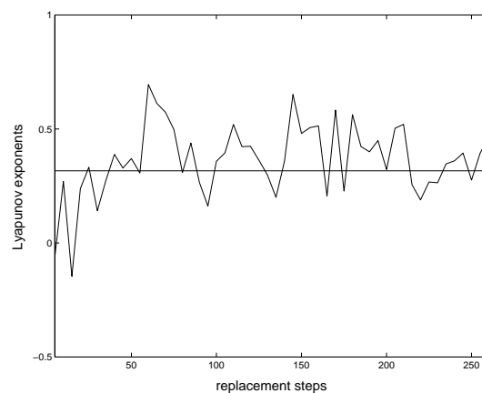
Figure 9. Evolution of the Lyapunov exponent with respect to replacement steps with low pass filtering.
