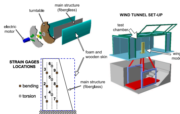
Figure 1. Experimental set-up and strain gages locations.
