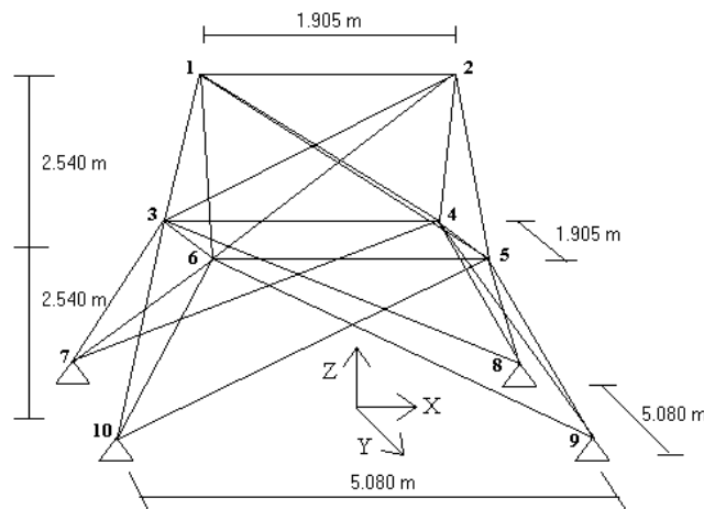
Figure 4. Sketch of the 25-bar space truss
