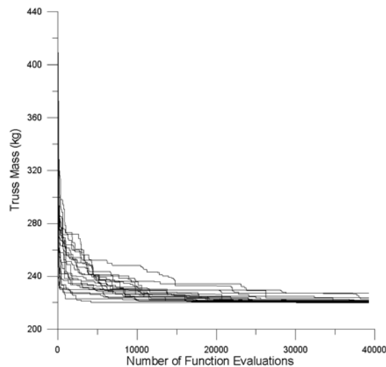
Figure 6. Best value of truss mass as a function of number of evaluations for 20 independent runs of GEO.
