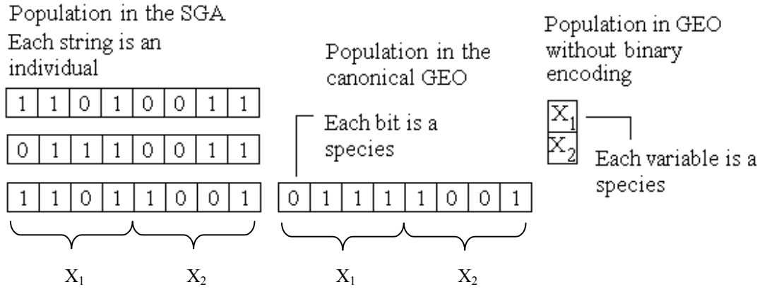
Figure 2. Population as represented in the SGA and GEO for a problem with 2 variables. In this example the population of the SGA has three individuals, while in the canonical GEO has 8 species and 2 species in GEO without binary encoding. For the SGA and the canonical GEO, each variable is encoded in 4 bits.
