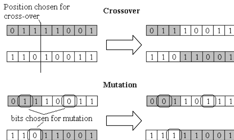
Figure 1. Outline of crossover and mutation in a Simple Genetic Algorithm
