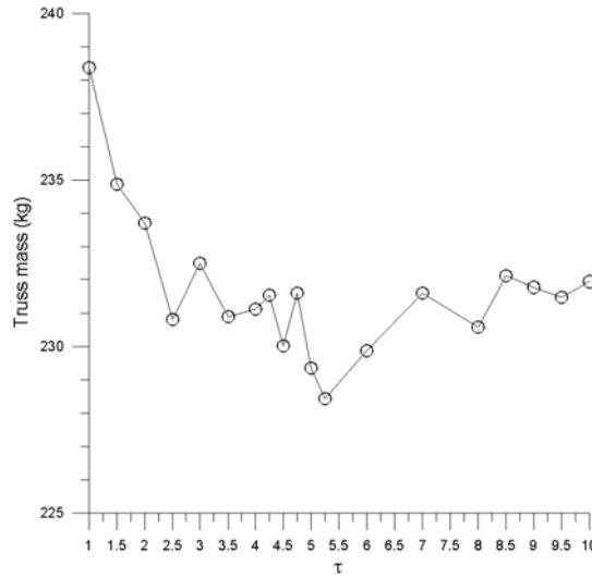
Figure 5. Average of the best values of the objective function in 20 runs for each value of \tau .
