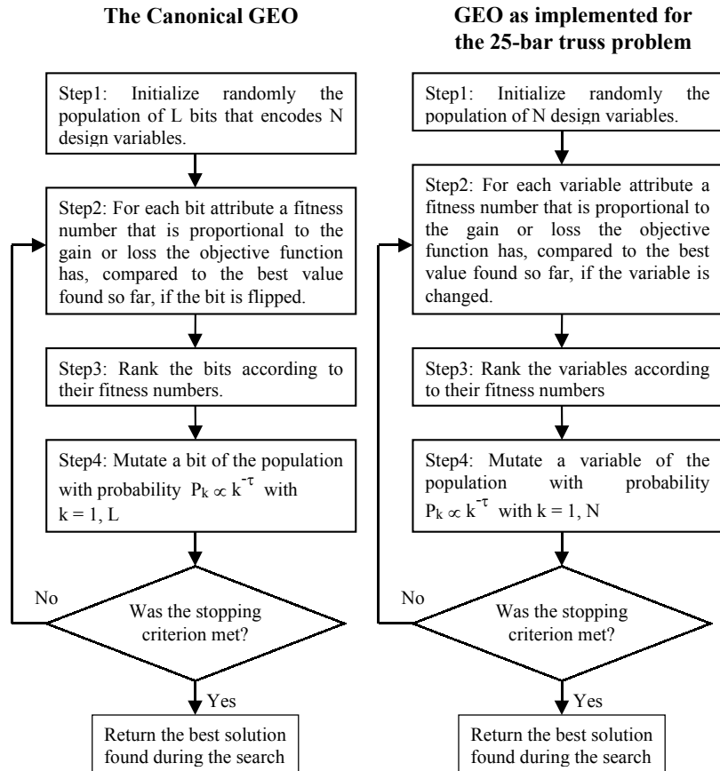
Figure 3. Main steps of the canonical GEO and its implementation for the 25-bar truss optimization problem
