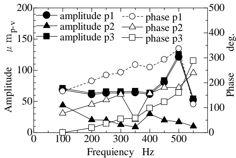
Figure 6. Amplitude and phase of sinusoidal motion at point p1-p3
