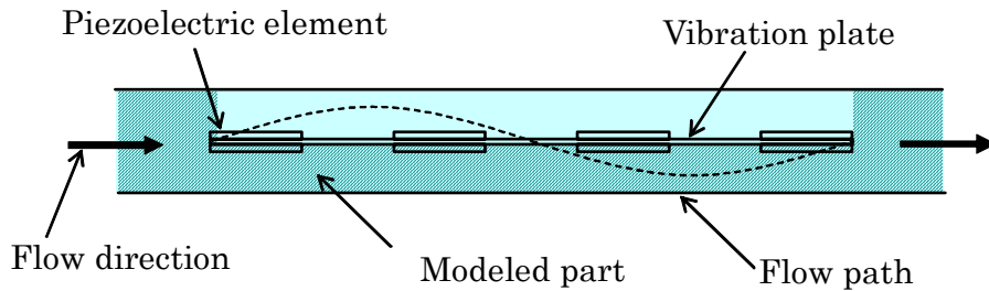
Figure 9. Schematic view of flow path cross section
