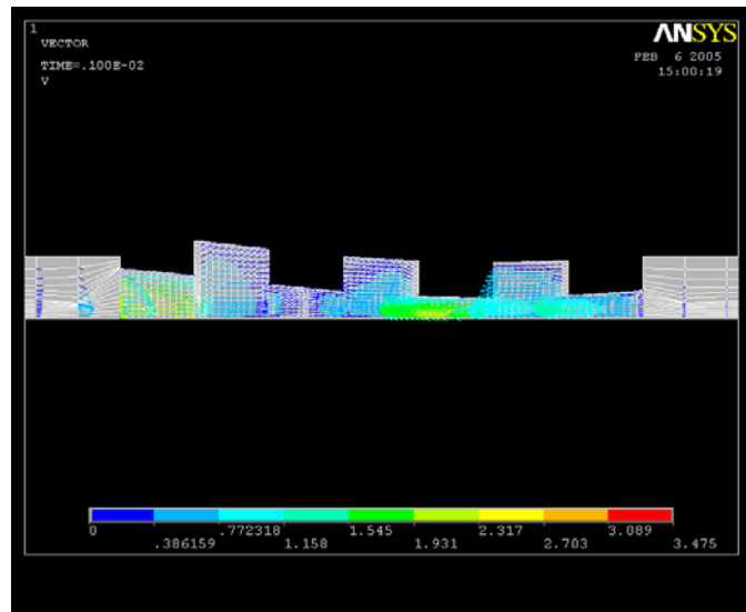
Figure 10. Example of simulation result image (flow velocity vector)
