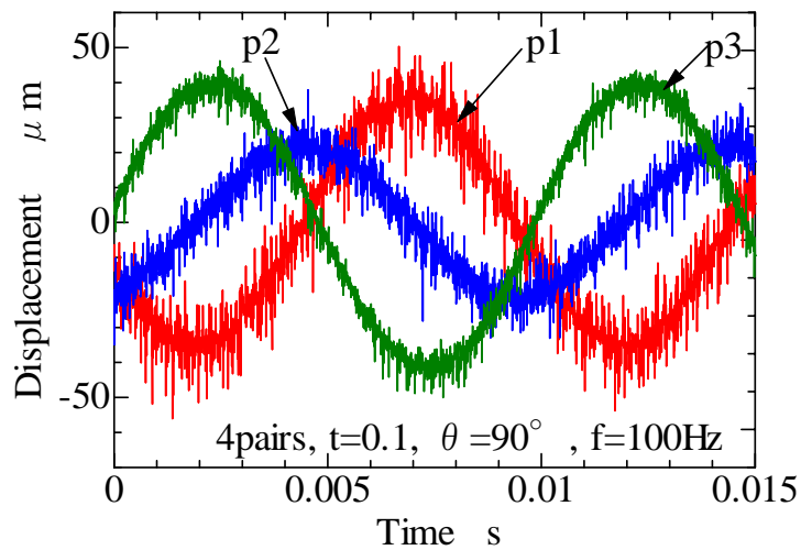
Figure 5. Behavior of vibration plate ( f=100\text{Hz} , \theta=90^\circ )
