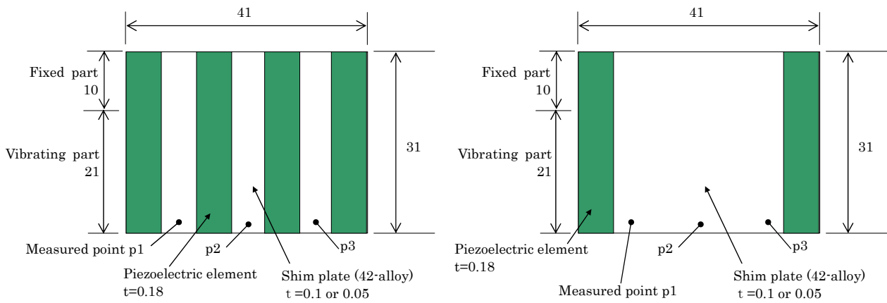
(a) Four series type vibration plate
