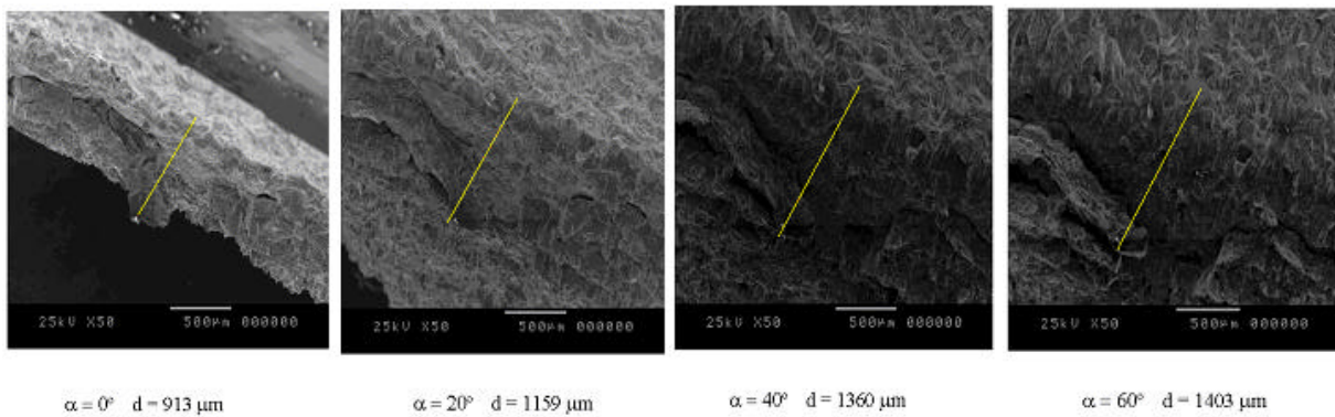
Figure 7. Measures of d for several inclination angles of the specimen ( T = -196^{\circ}\text{C} ).
