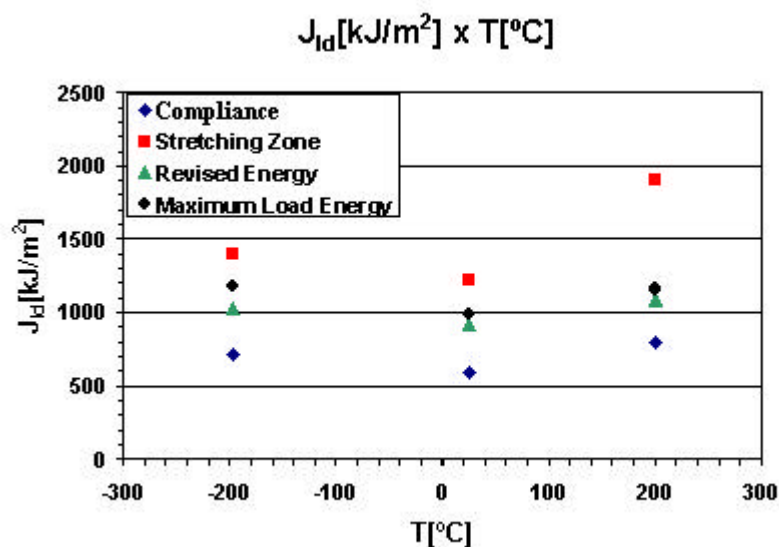
Figure 7. J_{Id} changing with temperature for different methods.
