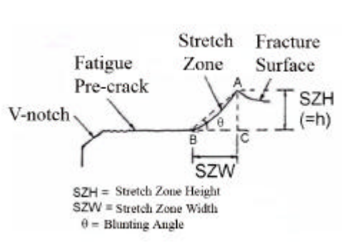
Figure 1. Profile of the stretching zone. Source: SREENIVASAN, 1996.
