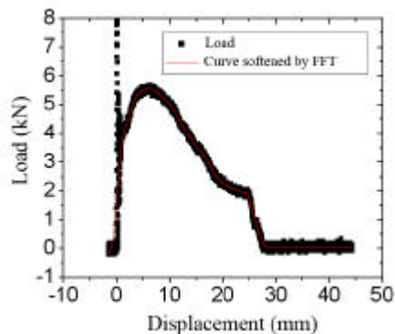
Figure 3. Curve smoothed by FFT, T = 200^{\circ}\text{C} .
