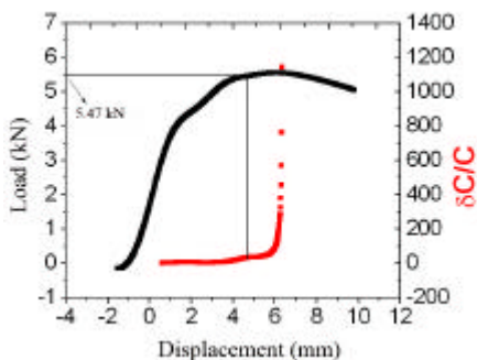
Figure 4. Variation of Compliance, T=200^{\circ}\text{C} .
