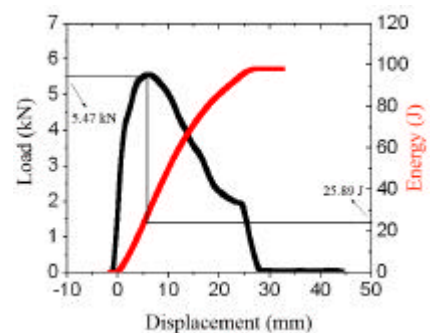
Figure 5. Energy associated to the beginning of the abrupt variation. T=200^{\circ}\text{C} .
