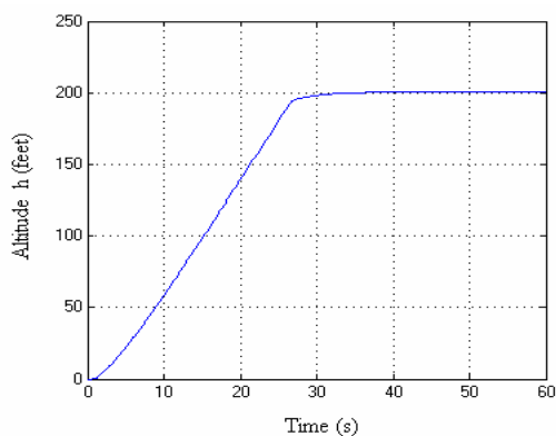
Figure 7. Response to altitude for continuous digital controller implemented in MATLAB/SIMULINK.
