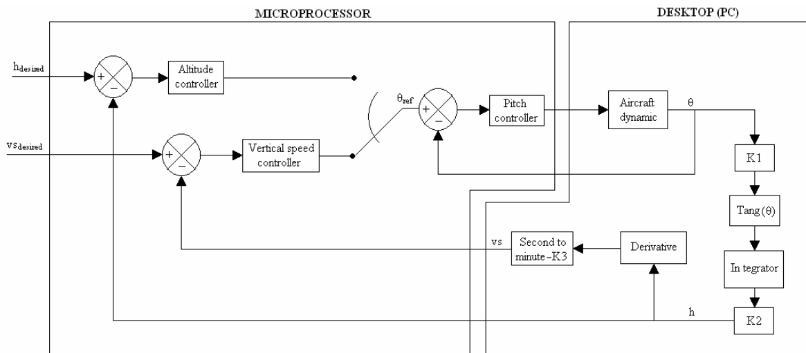
Figure 1. Block Diagram of the proposed longitudinal autopilot
