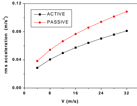
Figure 3: Root mean square acceleration of mass m_1 .
