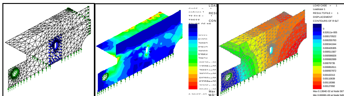
Figure 3 - Loading, stress, and displacement distribution for the hydraulic cylinder support.
