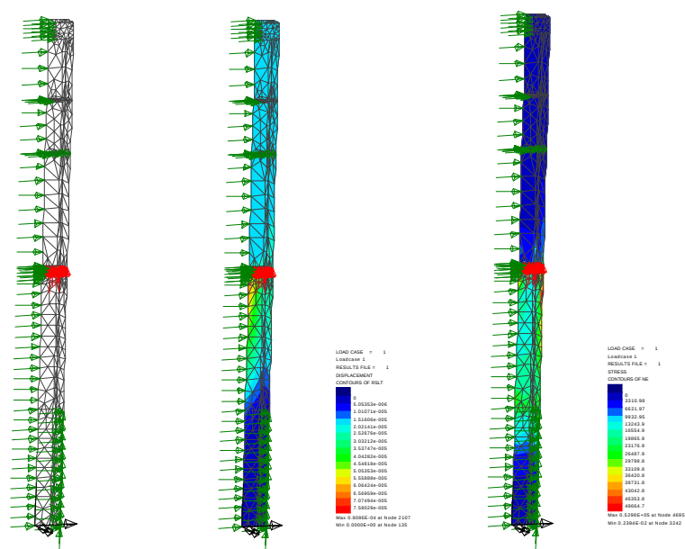
Figure 4 – Loading, displacement and stress distribution for columns beams.
