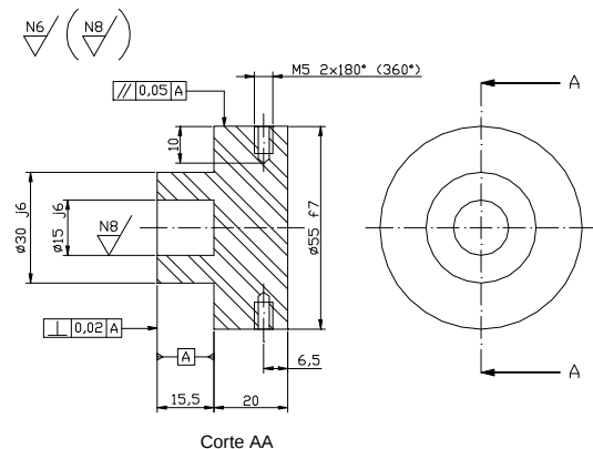
Figure 10: Indenter punch
