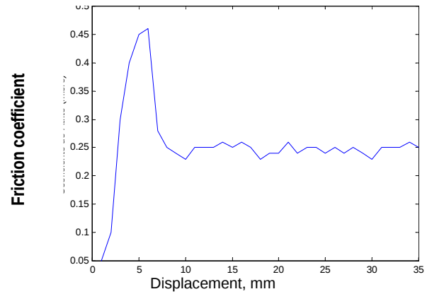
Figure 14 : Friction coefficient vs. Displacement Fn = 190,3 N
