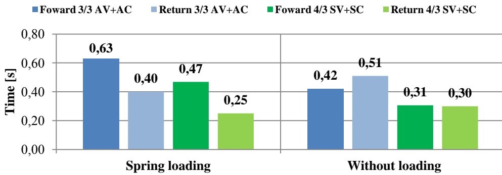
Figure 6. Rise time as a function of load and cylinder movement direction.
