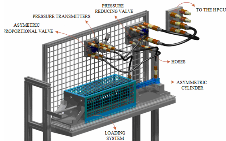
Figure 3. Workbench with a combination of asymmetric cylinder and asymmetric valve (SZPAK, 2008).
