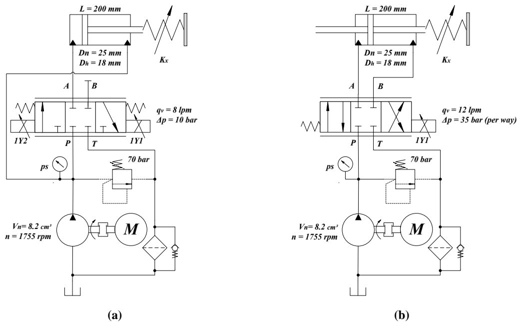
Figure 2. Electro-hydraulic circuits for positioning control: a) 3/3 AV+AC; b) 4/3 SV+SC.
