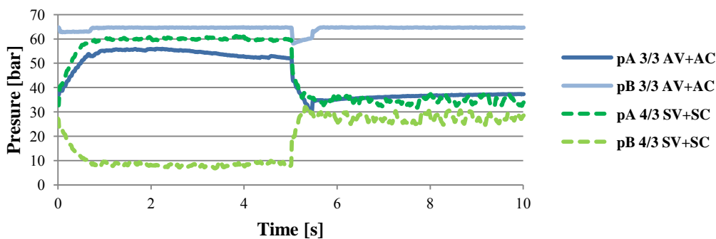
Figure 7. Pressure curves for the electro-hydraulic positioning systems with load.
