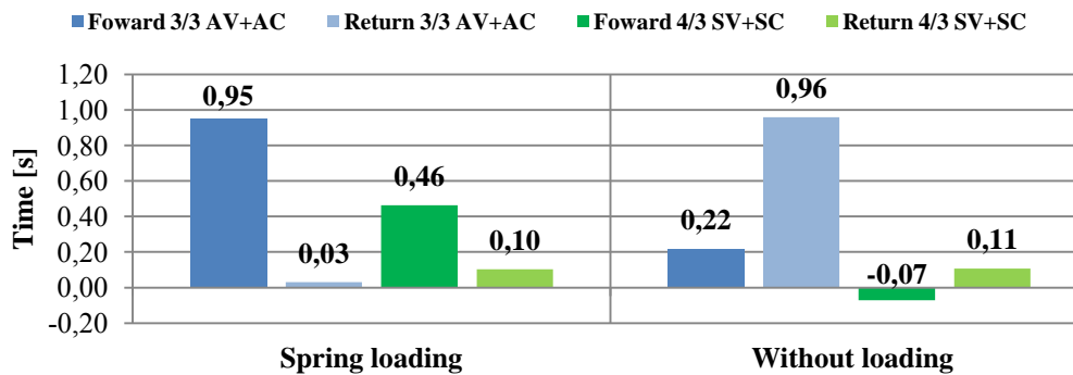
Figure 9. Steady state error of the settings studied as a function of load and cylinder movement.
