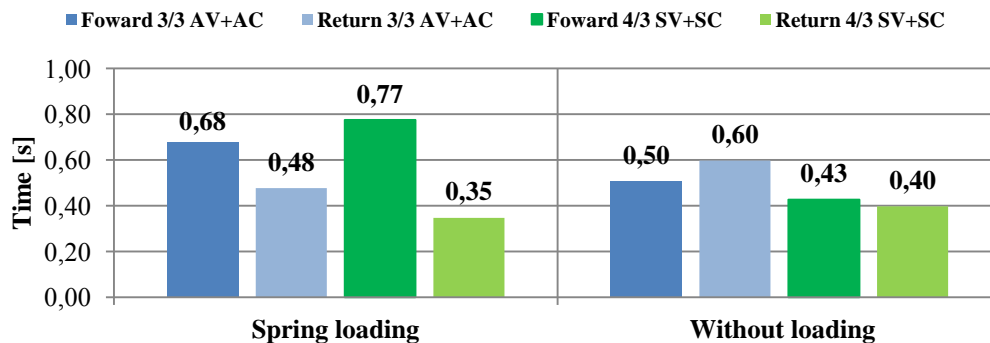
Figure 8. Settling time as a function of load and cylinder movement direction.
