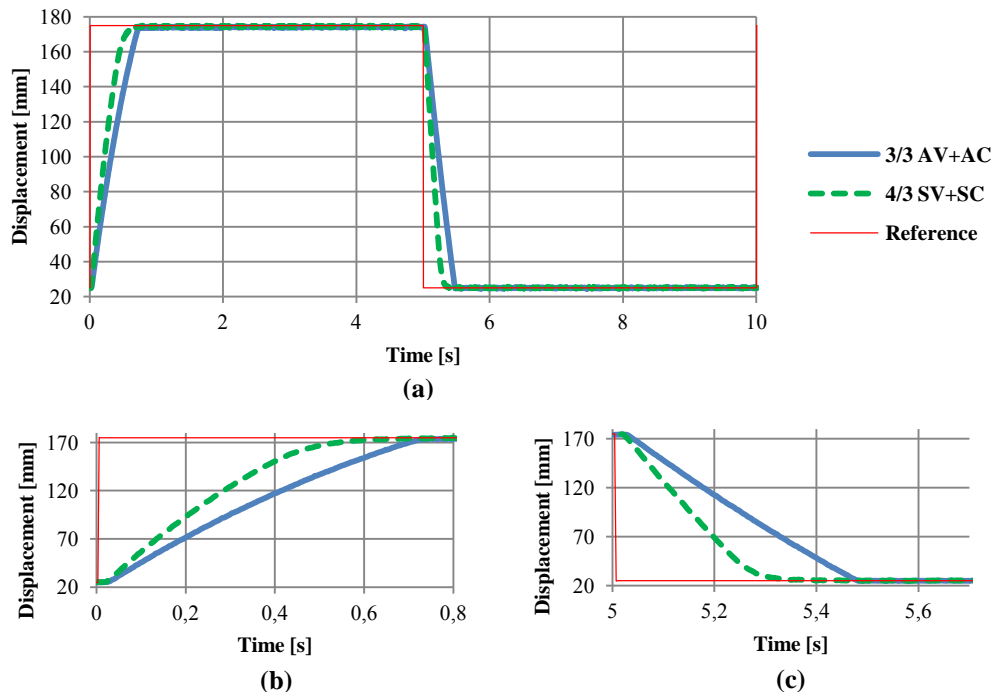
Figure 5. Position time response of the system with loading: (a) Complete cycle, (b) Forward direction, and (c) Return direction.
