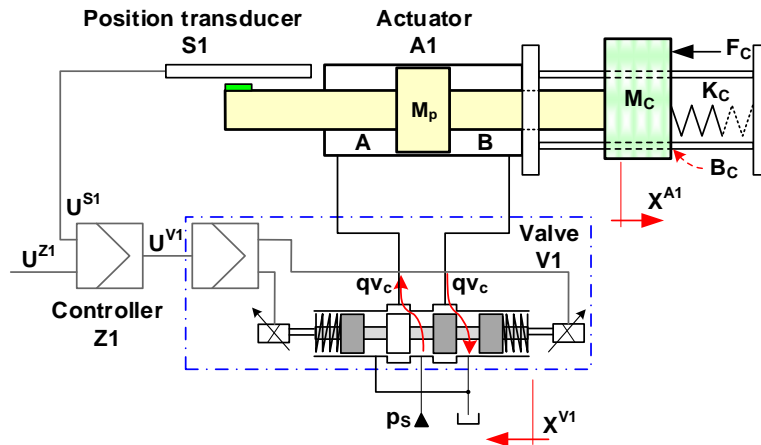
Figure 1. Electro-hydraulic system of positioning control (DE NEGRI, 2001).
