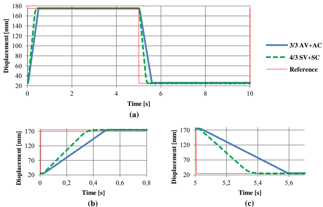
Figure 4. Position time response of the system without load: (a) Complete cycle, (b) Forward direction, and (c) Return direction.
