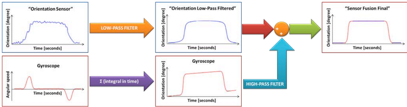
Figure 14. Example of the application of the complementary filter.
