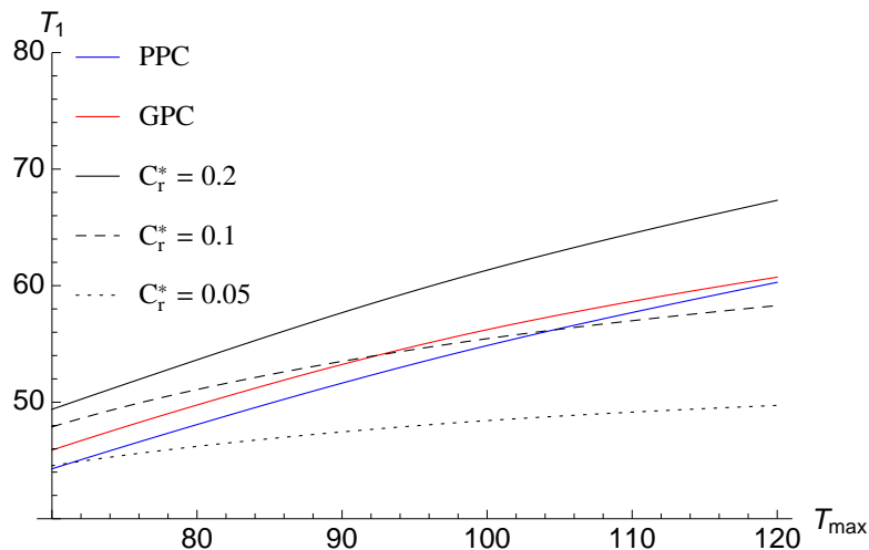
Figure 3. Variation of process side outlet temperature with regeneration temperature calculated with the algebraic correlation (PPC and GPC) and the PDE model (for different C_{r,j}^* values).
