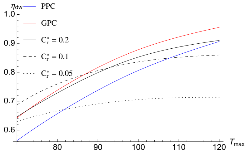
Figure 1. Variation of dehumidification efficiency with heat capacity ratio for different regeneration temperatures.
