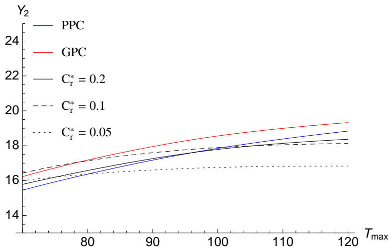
Figure 6. Variation of regeneration side outlet humidity ratio with regeneration temperature calculated with the algebraic correlation (PPC and GPC) and the PDE model (for different C_{r,j}^* values).
