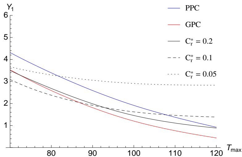
Figure 4. Variation of process side outlet humidity ratio with regeneration temperature calculated with the algebraic correlation (PPC and GPC) and the PDE model (for different C_{r,j}^* values).
