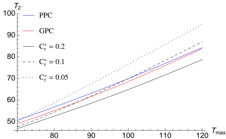
Figure 5. Variation of regeneration side outlet temperature with regeneration temperature calculated with the algebraic correlation (PPC and GPC) and the PDE model (for different C_{r,j}^* values).
