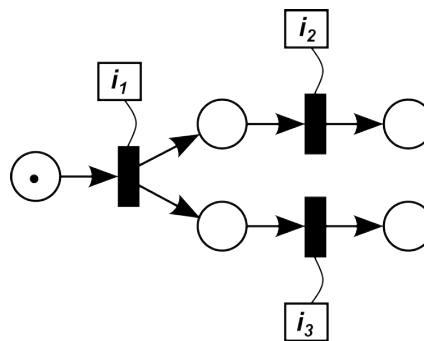
Figure 6: Instructions parallelism in PPN
