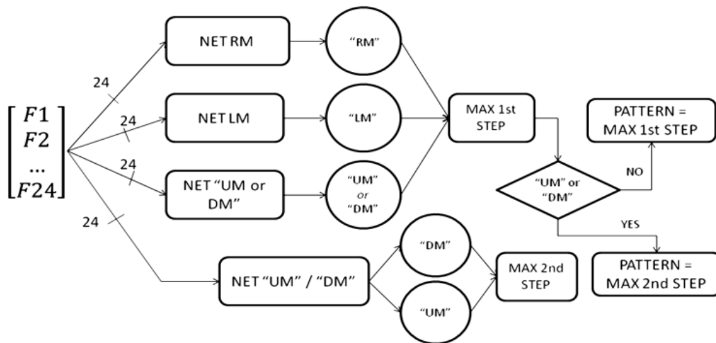
Figure 7. Hierarchical model.
