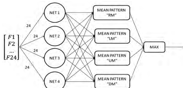
Figure 5. Ensemble model.
