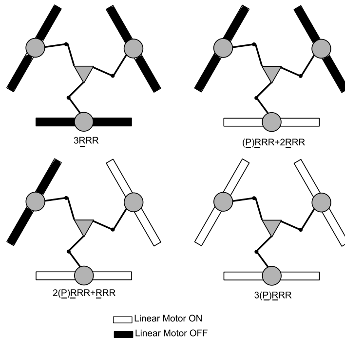
Figure 2. 3R\underline{R}R : planar parallel manipulator, (P)\underline{R}R\underline{R}R+2\underline{R}R\underline{R}R : one redundant actuator, 2(P)\underline{R}R\underline{R}R+\underline{R}R\underline{R}R : two redundant actuators and 3R\underline{R}R : three redundant actuators
