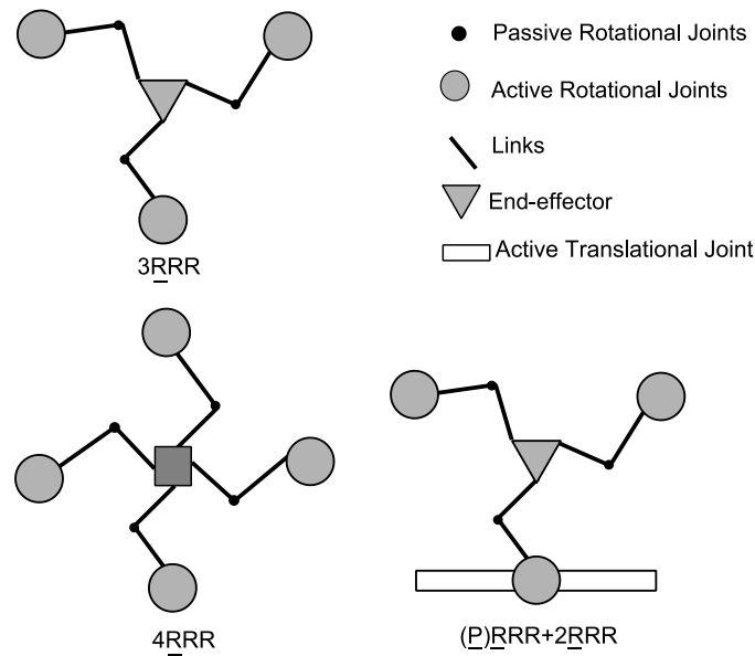
Figure 1. 3R\underline{R}R : planar parallel manipulator, 4R\underline{R}R : redundant actuated planar manipulator and (P)R\underline{R}R\underline{R}R+2R\underline{R}R\underline{R}R : planar kinematically redundant planar manipulator
