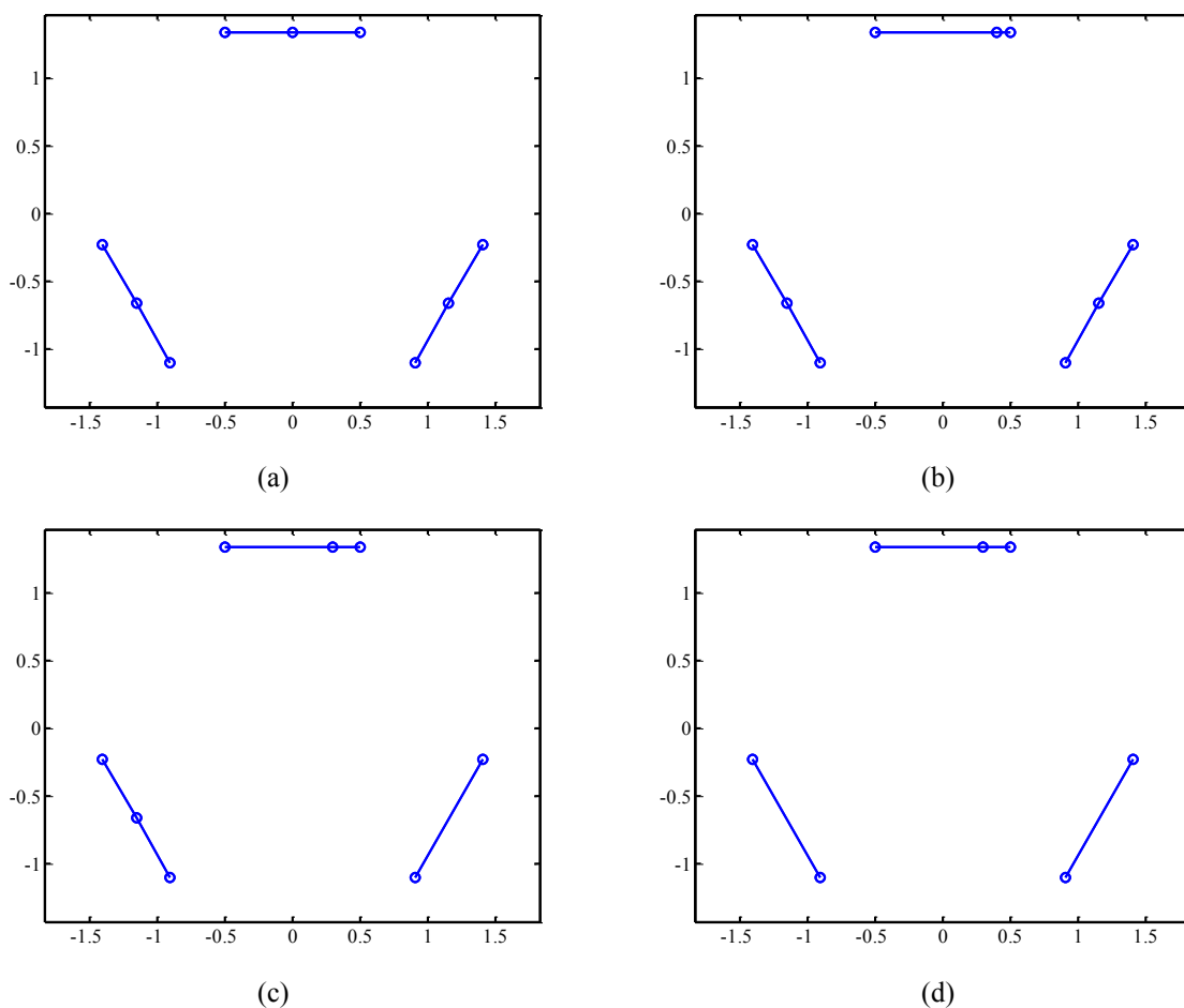
Figure 9. The best configuration of the (a) 3\underline{RRR} , (b) (\underline{P})\underline{RRR}+2\underline{RRR} , (c) 2(\underline{P})\underline{RRR}+\underline{RRR} and (d) 3(\underline{P})\underline{RRR}+2\underline{RRR}
