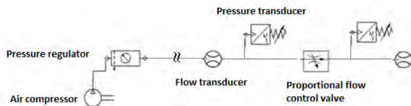
Figure 2. Valve test.
