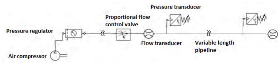
Figure 4. Pipeline test.
