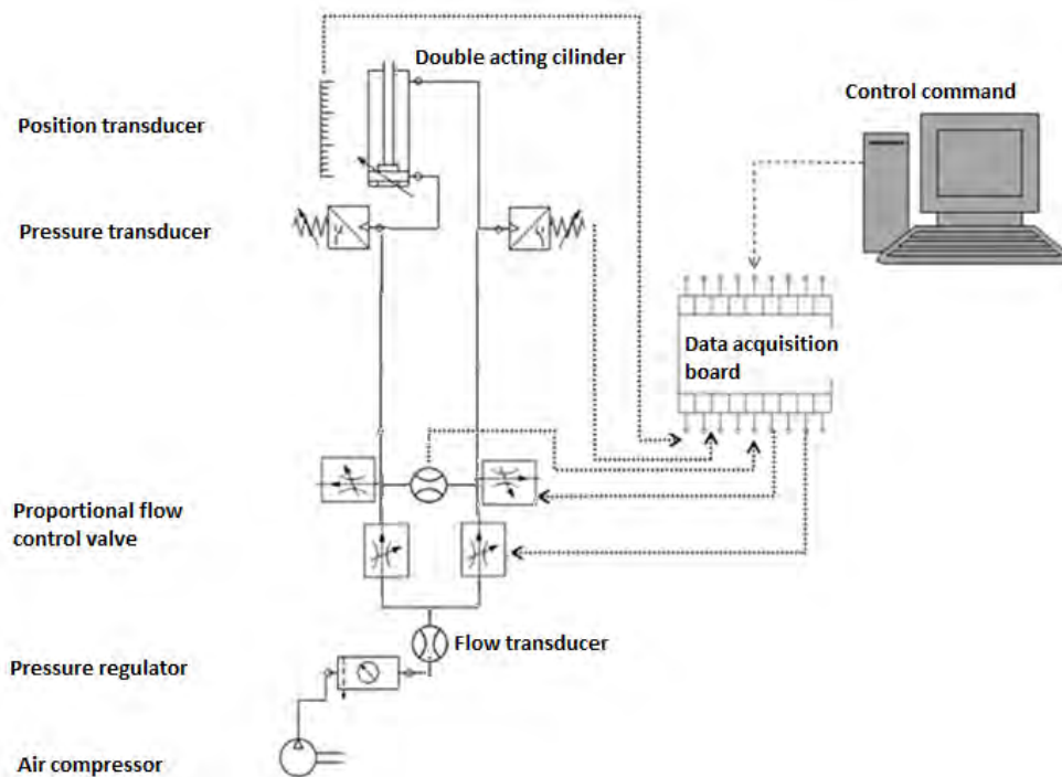
Figure 1. Test rig.
