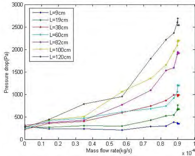
Figure 5. Pressure drop in pipelines of different length.
