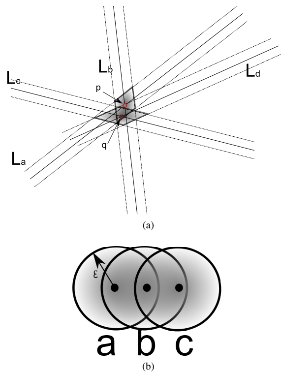
Figure 2. Floating point arithmetic problems. (a) Asymmetric incidence problem. (b) Incidence intransitivity.
