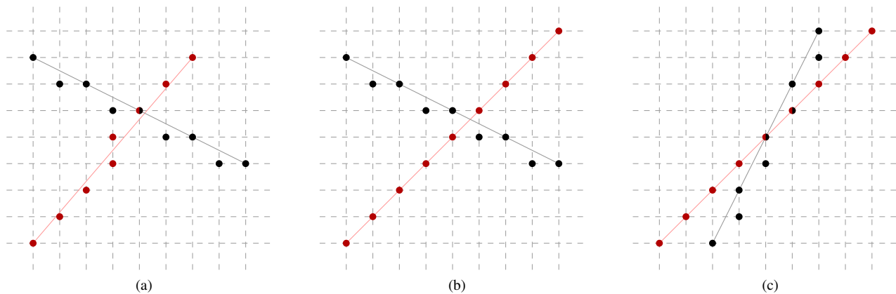
Figure 8. Bresenham generated lines intersection. (a) One point in common; (b) no common point between line segments; (c) multiple common points.
