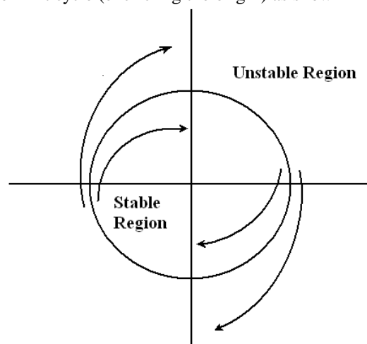
Figure 3. Unstable Limit Cycle.
