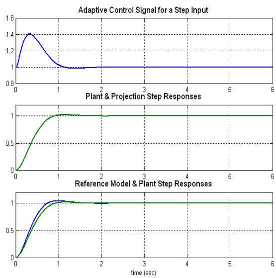
Figure 6b. DMRAC Closed Loop Response for J=0.01 .
