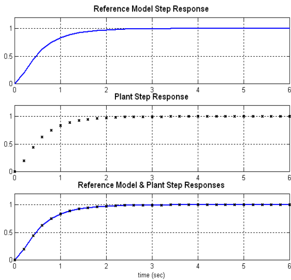
Figure 4. Reference Model and Plant at Model Matching Conditions.
