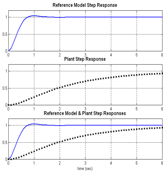
Figure 10a. Plant Open Loop Response for J=0.20 .
