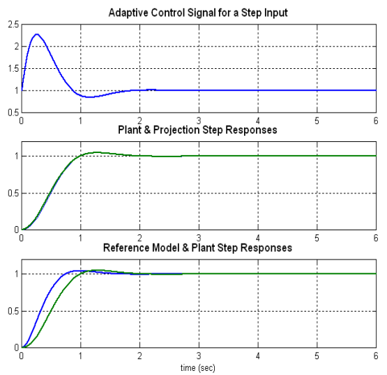
Figure 7b. DMRAC Closed Loop Response for J=0.05 .
