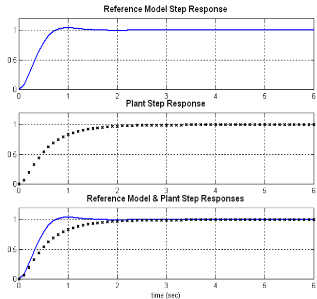
Figure 5. Reference Model Specification for Design Purposes.
