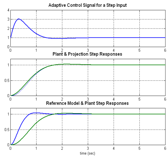
Figure 9b. DMRAC Closed Loop Response for J=0.15 .
