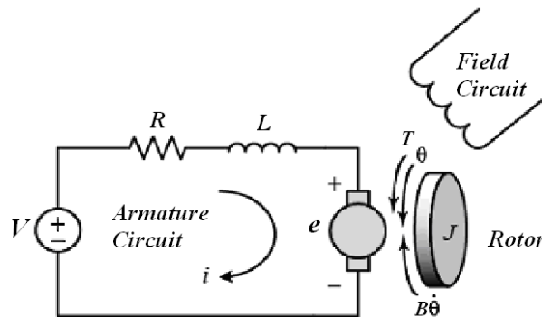
Figure 1. The DC Motor.
