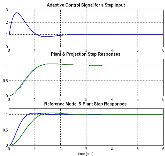
Figure 8b. DMRAC Closed Loop Response for J=0.10 .
