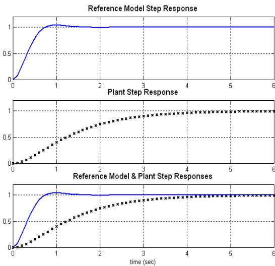
Figure 8a. Plant Open Loop Response for J=0.10 .
