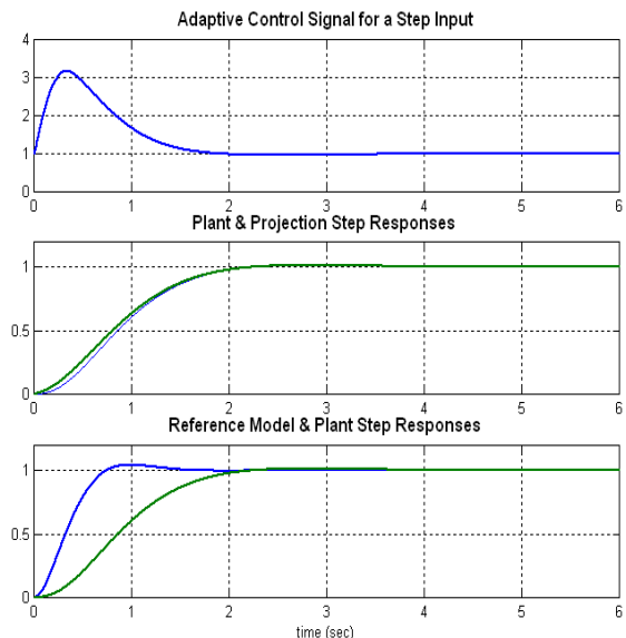
Figure 10b. DMRAC Closed Loop Response for J=0.20 .
