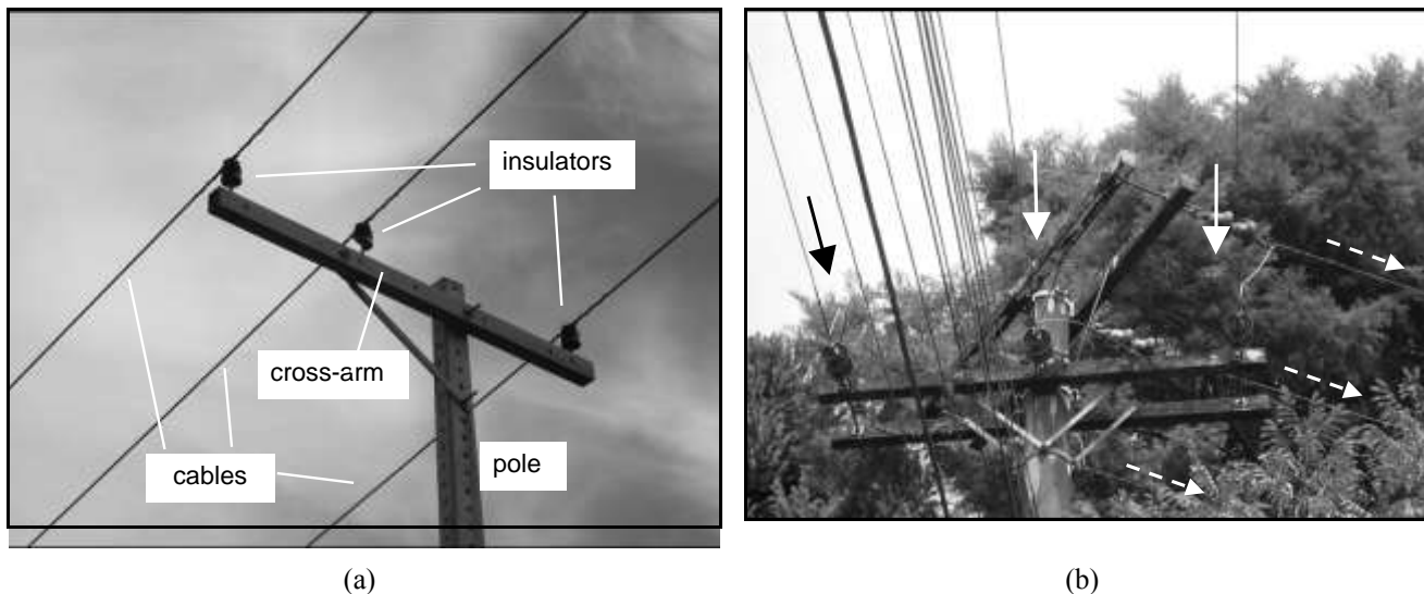
Figure 1. Usual electrical distribution lines. (a) Simple path, (b) Complex path.
