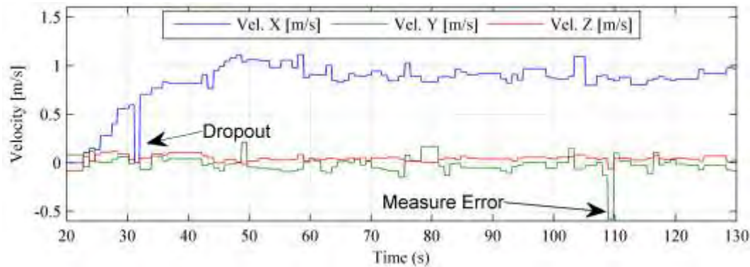
Figure 13. Velocity DVL measurements of the Pirajuba DVL in an acceleration phase of a zigzag manoeuvre.
