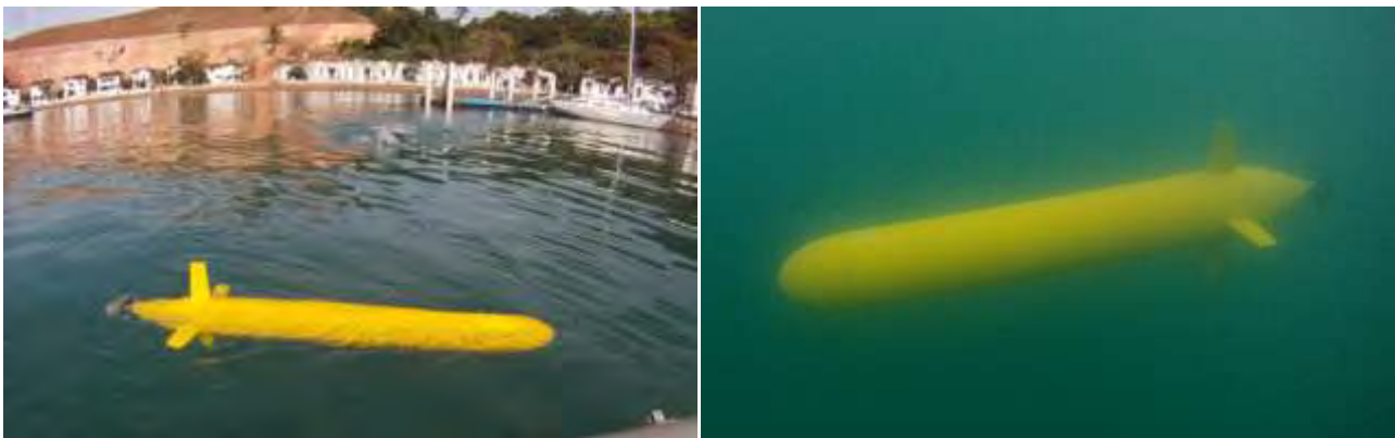
Figure 1. Pirajuba AUV during the identification tests.
